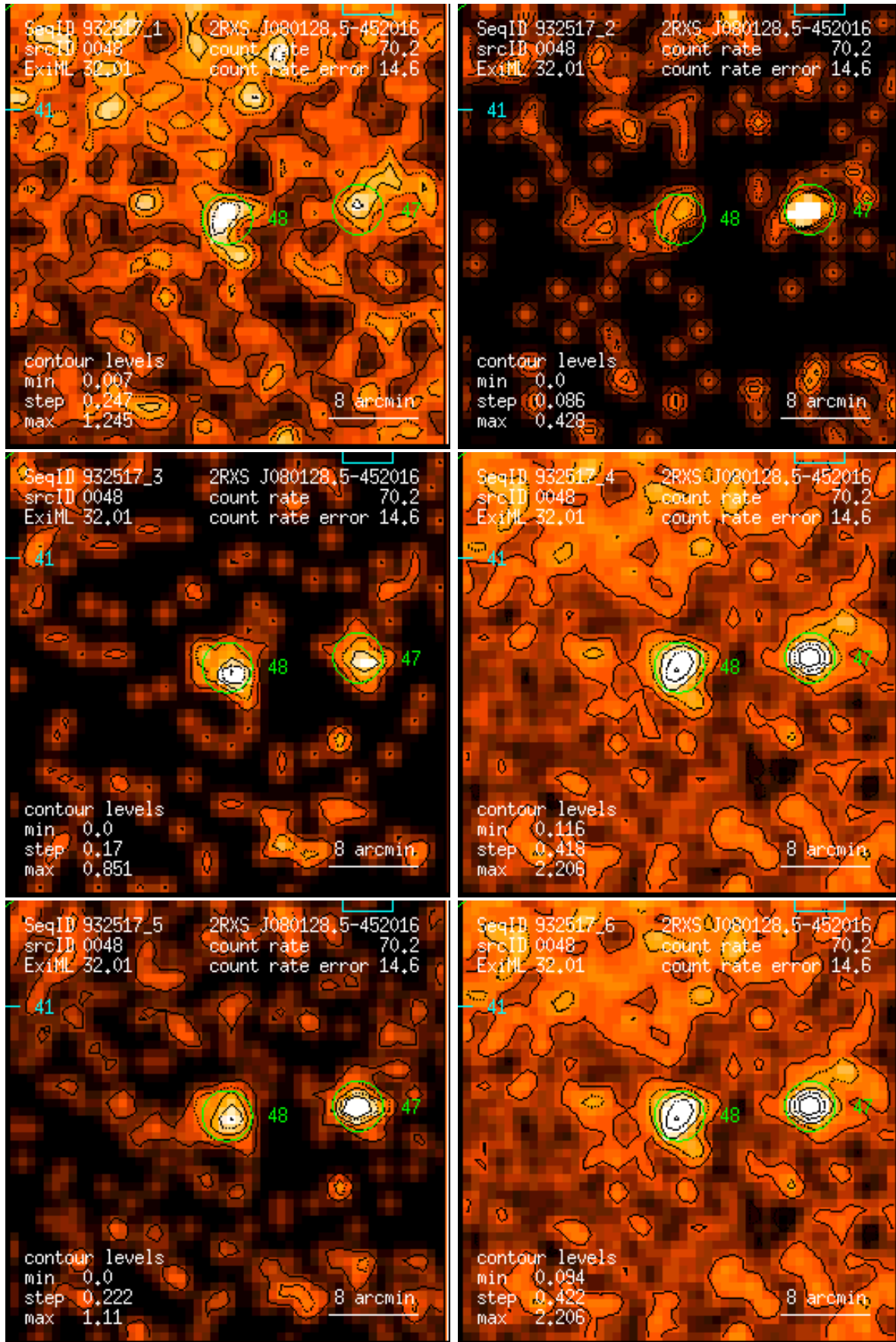
Figure 48: RASS 932517: detection 0048: band rate images, Gaussian filter: (1) PSPC channels 11 – 41, (2) 52 – 90, (3) 91 – 201, (4) 11 – 235, (5) 52 – 201, (6) 11 – 201. Broad band rates in counts/ks. Band rate contour levels in counts/ks/arcmin 2 .
