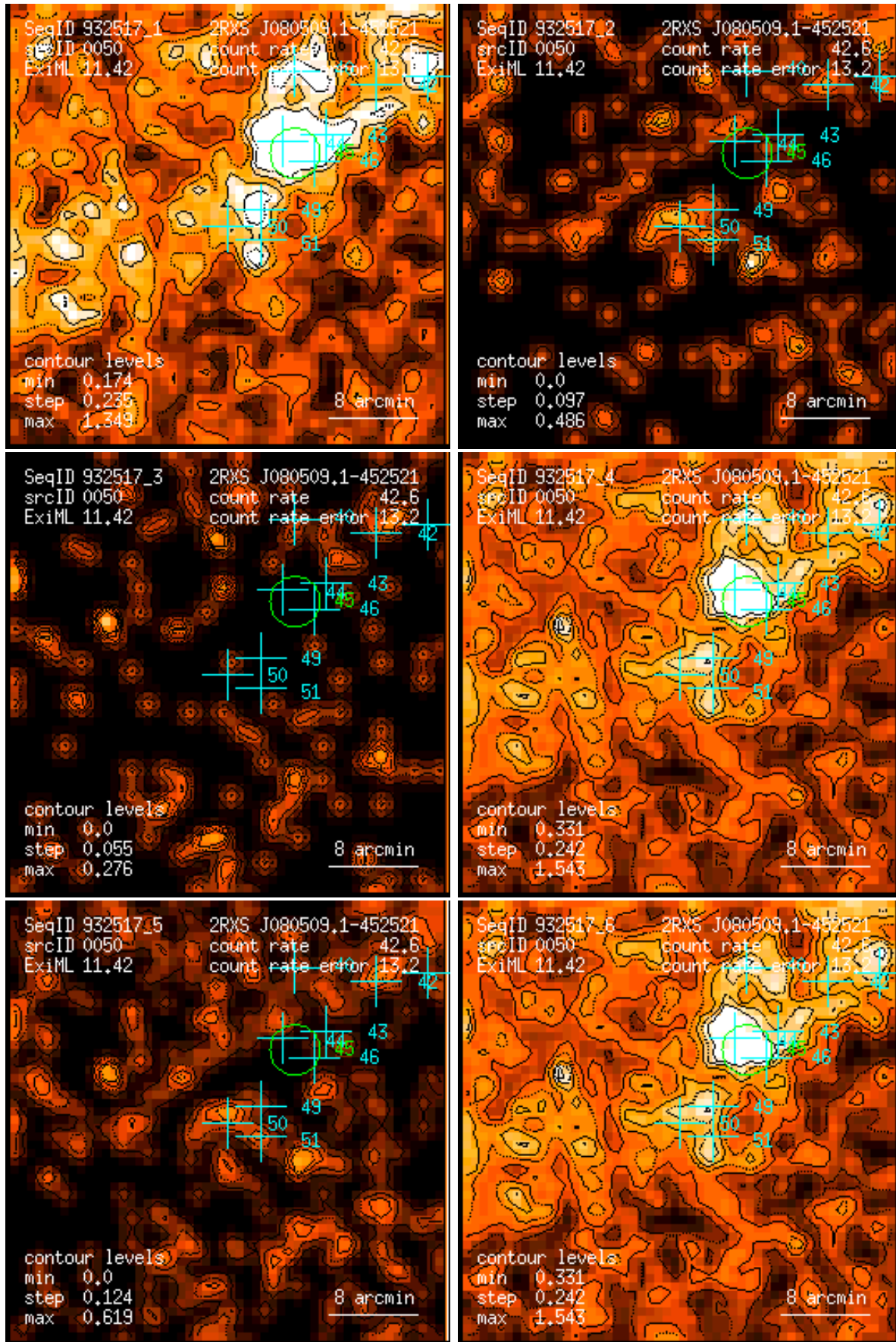
Figure 50: RASS 932517: detection 0050: band rate images, Gaussian filter: (1) PSPC channels 11 – 41, (2) 52 – 90, (3) 91 – 201, (4) 11 – 235, (5) 52 – 201, (6) 11 – 201. Broad band rates in counts/ks. Band rate contour levels in counts/ks/arcmin 2 .
