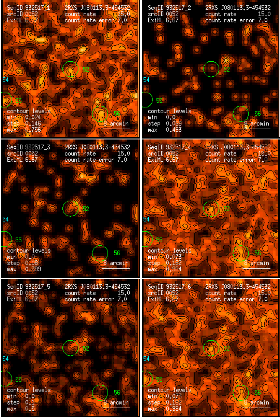
Figure 52: RASS 932517: detection 0052: band rate images, Gaussian filter: (1) PSPC channels 11 – 41, (2) 52 – 90, (3) 91 – 201, (4) 11 – 235, (5) 52 – 201, (6) 11 – 201. Broad band rates in counts/ks. Band rate contour levels in counts/ks/arcmin 2 .
