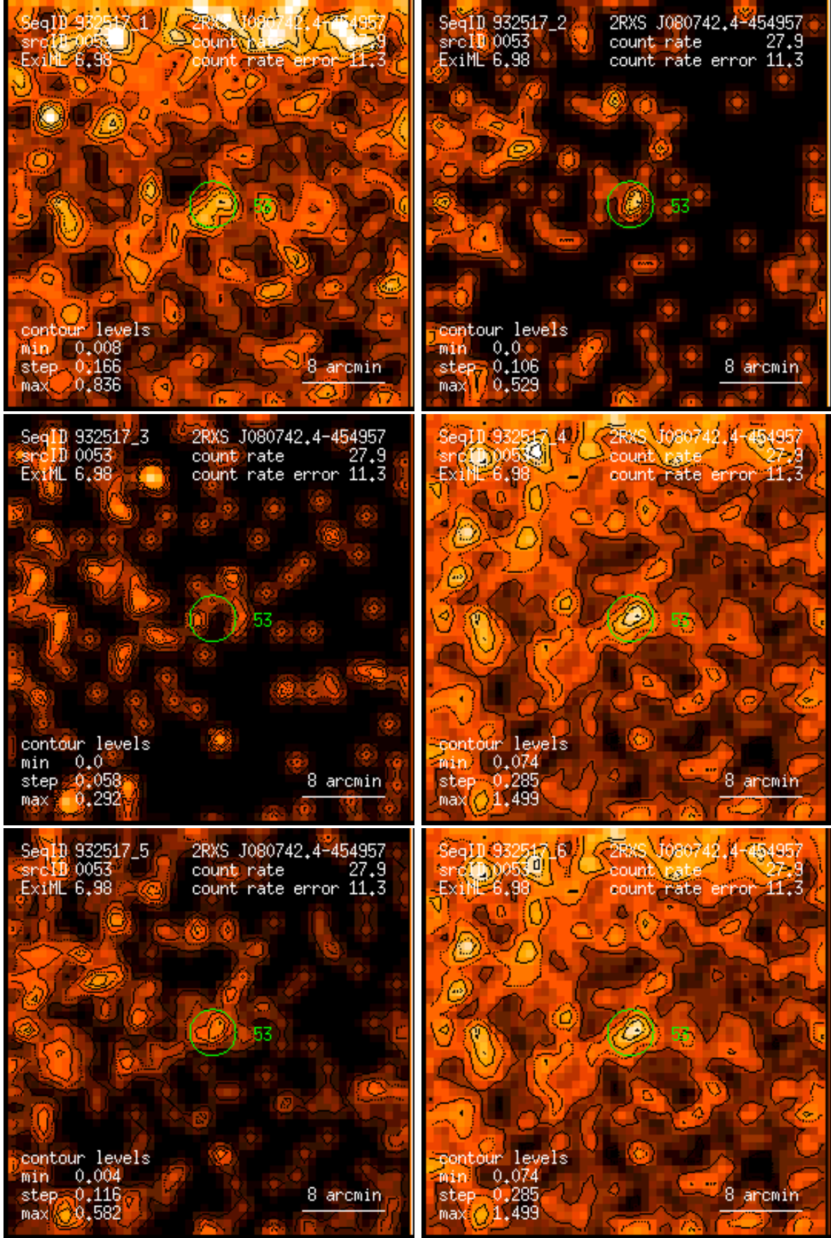
Figure 53: RASS 932517: detection 0053: band rate images, Gaussian filter: (1) PSPC channels 11 – 41, (2) 52 – 90, (3) 91 – 201, (4) 11 – 235, (5) 52 – 201, (6) 11 – 201. Broad band rates in counts/ks. Band rate contour levels in counts/ks/arcmin 2 .
