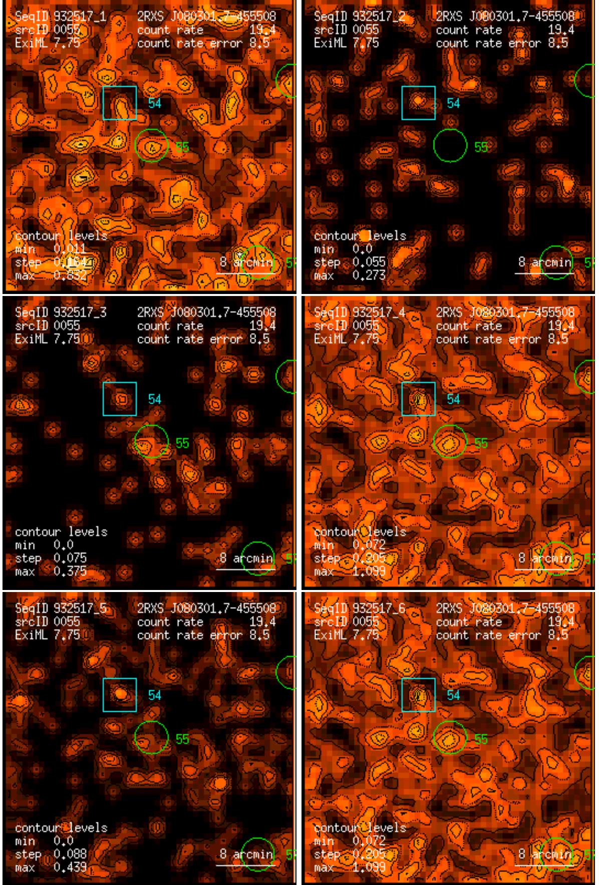
Figure 55: RASS 932517: detection 0055: band rate images, Gaussian filter: (1) PSPC channels 11 – 41, (2) 52 – 90, (3) 91 – 201, (4) 11 – 235, (5) 52 – 201, (6) 11 – 201. Broad band rates in counts/ks. Band rate contour levels in counts/ks/arcmin 2 .
