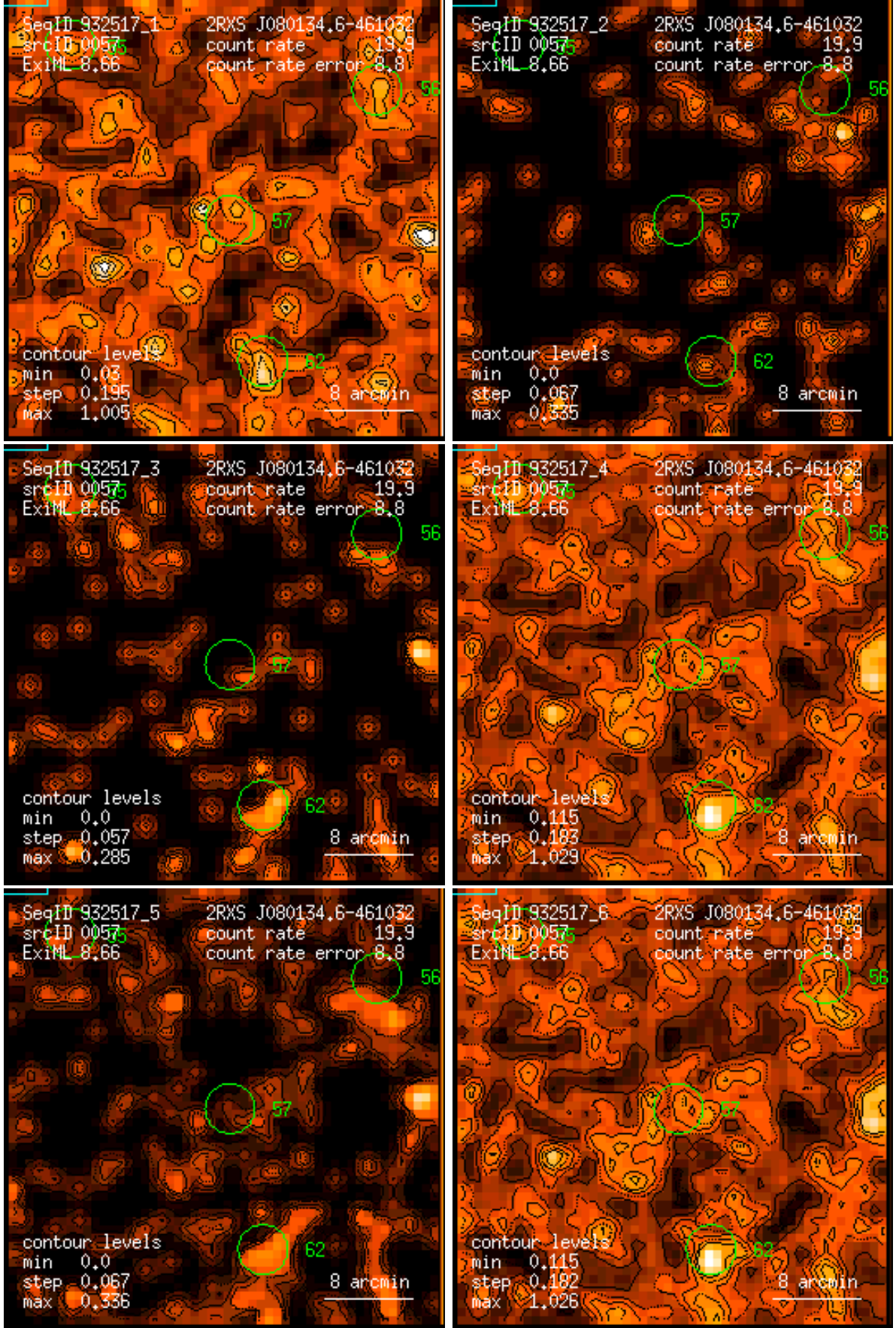
Figure 57: RASS 932517: detection 0057: band rate images, Gaussian filter: (1) PSPC channels 11 – 41, (2) 52 – 90, (3) 91 – 201, (4) 11 – 235, (5) 52 – 201, (6) 11 – 201. Broad band rates in counts/ks. Band rate contour levels in counts/ks/arcmin 2 .
