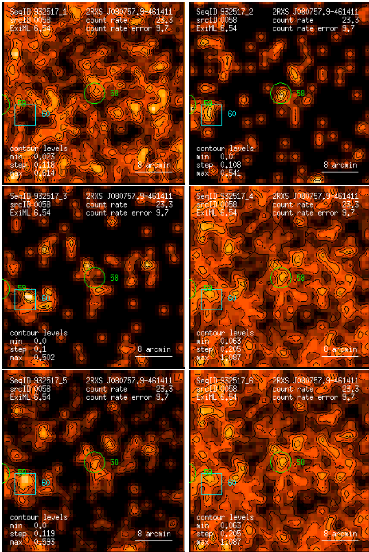
Figure 58: RASS 932517: detection 0058: band rate images, Gaussian filter: (1) PSPC channels 11 – 41, (2) 52 – 90, (3) 91 – 201, (4) 11 – 235, (5) 52 – 201, (6) 11 – 201. Broad band rates in counts/ks. Band rate contour levels in counts/ks/arcmin 2 .
