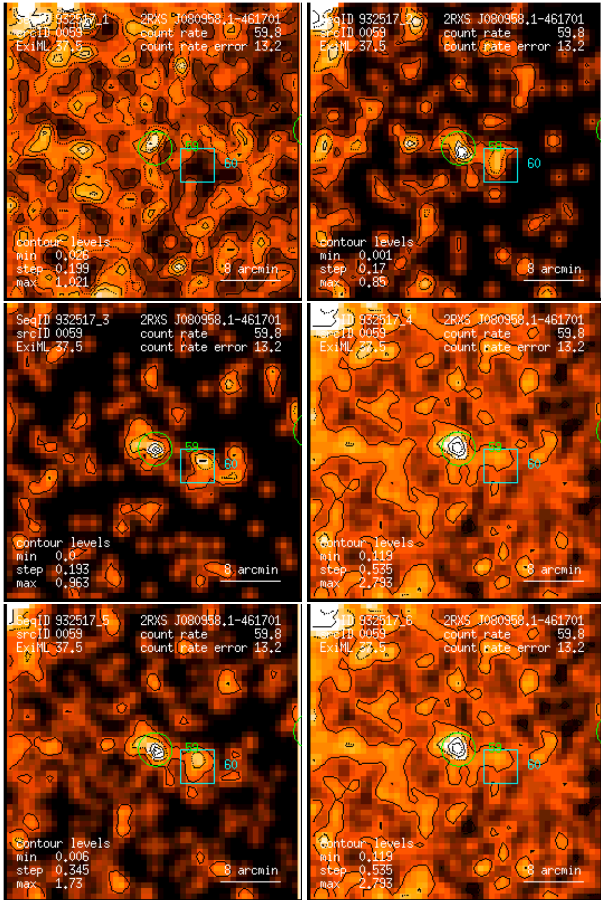
Figure 59: RASS 932517: detection 0059: band rate images, Gaussian filter: (1) PSPC channels 11 – 41, (2) 52 – 90, (3) 91 – 201, (4) 11 – 235, (5) 52 – 201, (6) 11 – 201. Broad band rates in counts/ks. Band rate contour levels in counts/ks/arcmin 2 .
