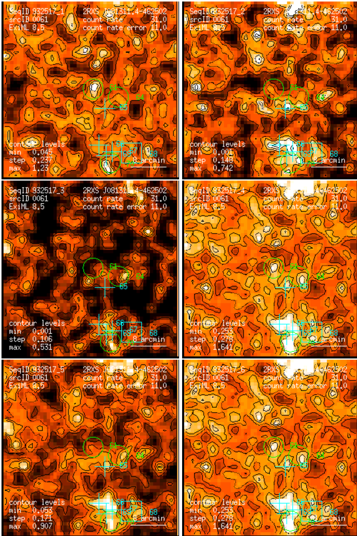
Figure 61: RASS 932517: detection 0061: band rate images, Gaussian filter: (1) PSPC channels 11 – 41, (2) 52 – 90, (3) 91 – 201, (4) 11 – 235, (5) 52 – 201, (6) 11 – 201. Broad band rates in counts/ks. Band rate contour levels in counts/ks/arcmin 2 .
