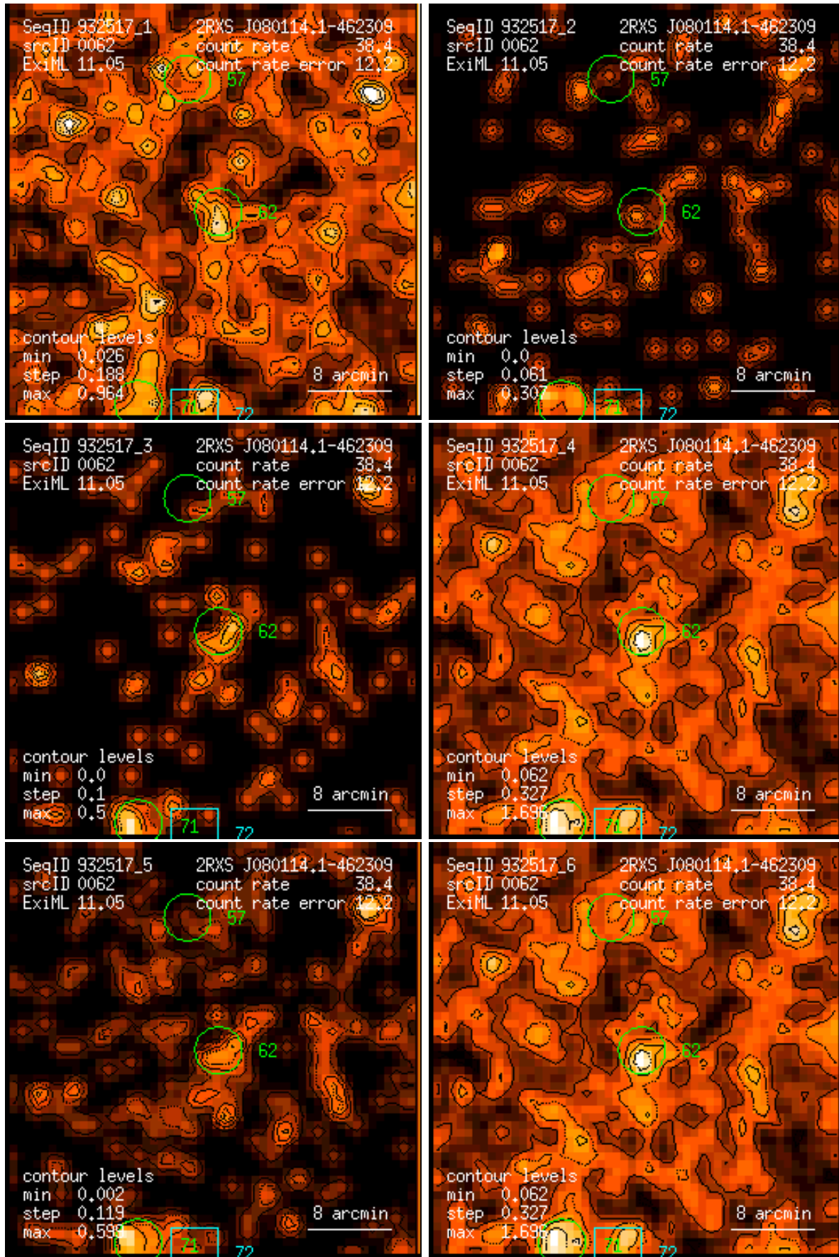
Figure 62: RASS 932517: detection 0062: band rate images, Gaussian filter: (1) PSPC channels 11 – 41, (2) 52 – 90, (3) 91 – 201, (4) 11 – 235, (5) 52 – 201, (6) 11 – 201. Broad band rates in counts/ks. Band rate contour levels in counts/ks/arcmin 2 .
