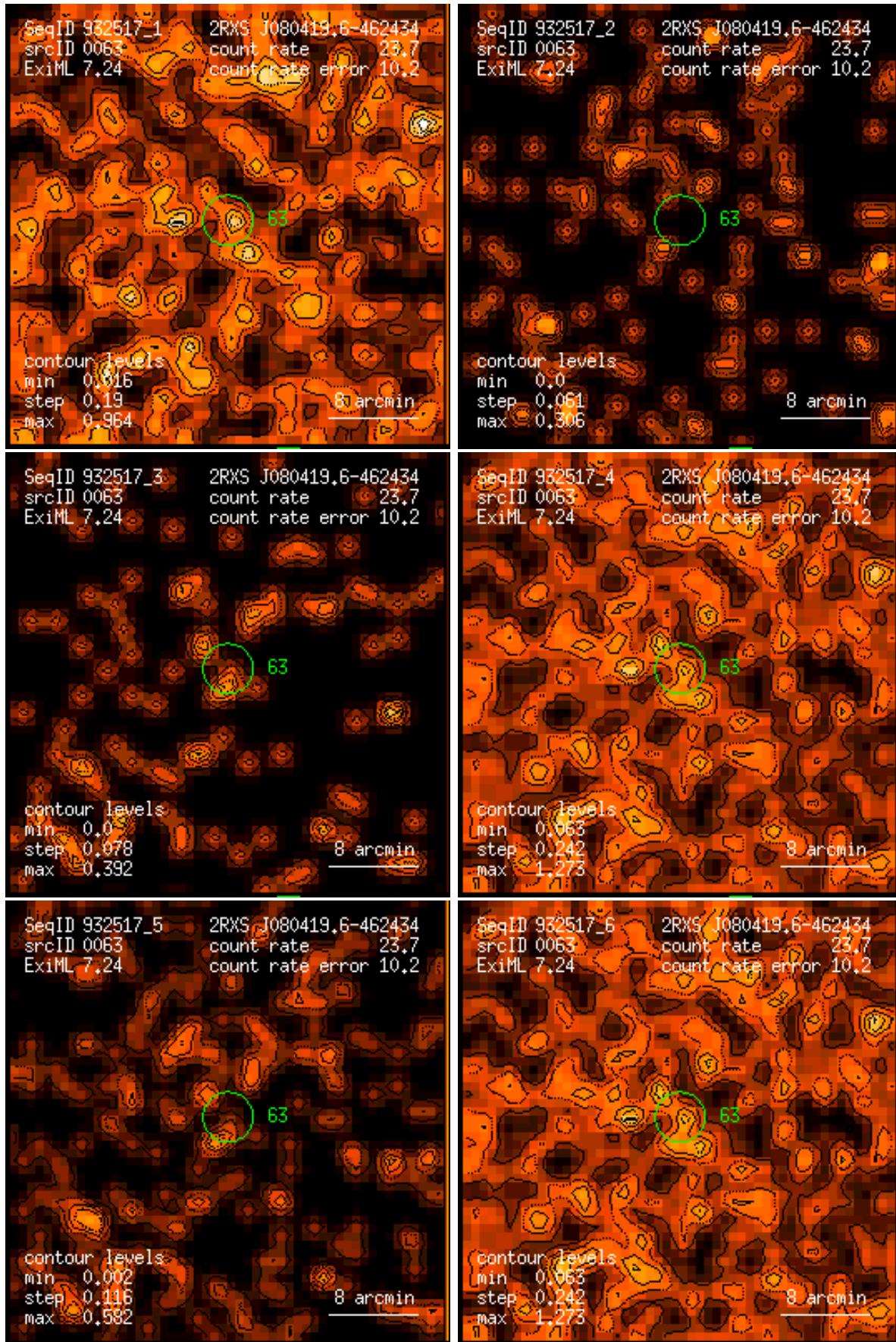
Figure 63: RASS 932517: detection 0063: band rate images, Gaussian filter: (1) PSPC channels 11 – 41, (2) 52 – 90, (3) 91 – 201, (4) 11 – 235, (5) 52 – 201, (6) 11 – 201. Broad band rates in counts/ks. Band rate contour levels in counts/ks/arcmin 2 .
