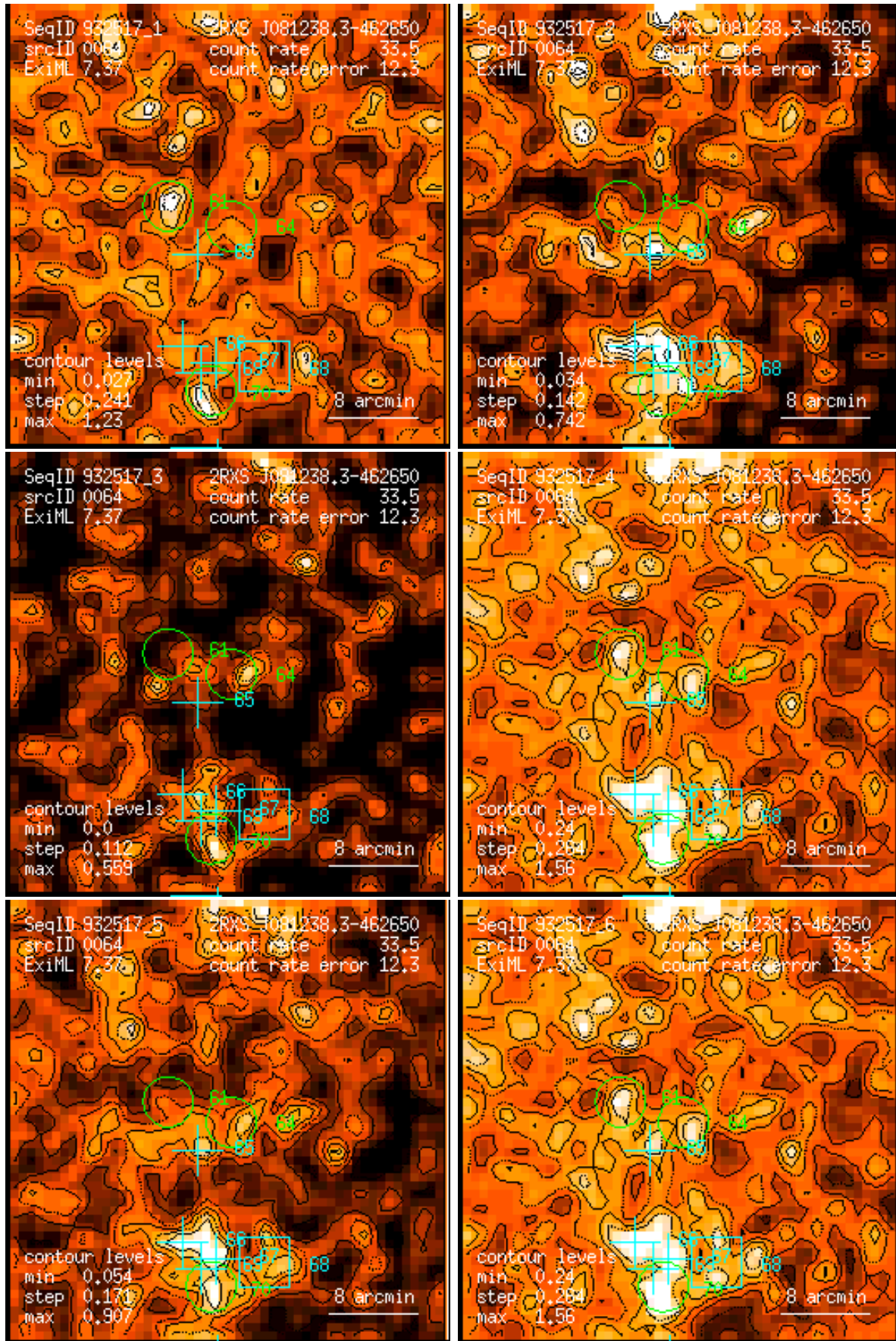
Figure 64: RASS 932517: detection 0064: band rate images, Gaussian filter: (1) PSPC channels 11 – 41, (2) 52 – 90, (3) 91 – 201, (4) 11 – 235, (5) 52 – 201, (6) 11 – 201. Broad band rates in counts/ks. Band rate contour levels in counts/ks/arcmin 2 .
