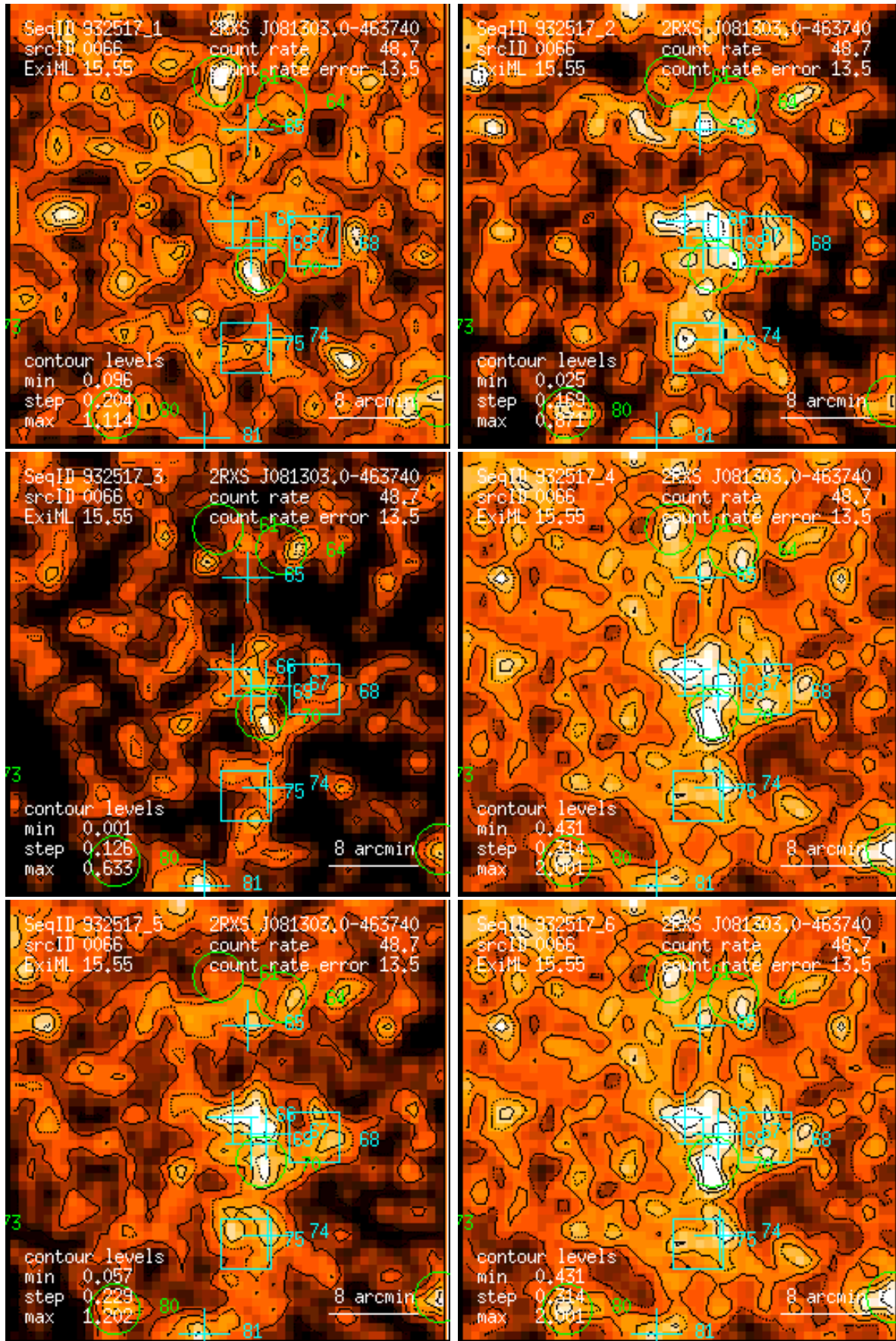
Figure 66: RASS 932517: detection 0066: band rate images, Gaussian filter: (1) PSPC channels 11 – 41, (2) 52 – 90, (3) 91 – 201, (4) 11 – 235, (5) 52 – 201, (6) 11 – 201. Broad band rates in counts/ks. Band rate contour levels in counts/ks/arcmin 2 .
