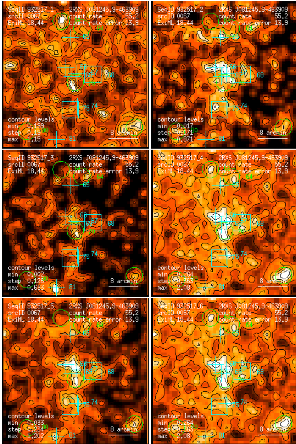
Figure 67: RASS 932517: detection 0067: band rate images, Gaussian filter: (1) PSPC channels 11 – 41, (2) 52 – 90, (3) 91 – 201, (4) 11 – 235, (5) 52 – 201, (6) 11 – 201. Broad band rates in counts/ks. Band rate contour levels in counts/ks/arcmin 2 .
