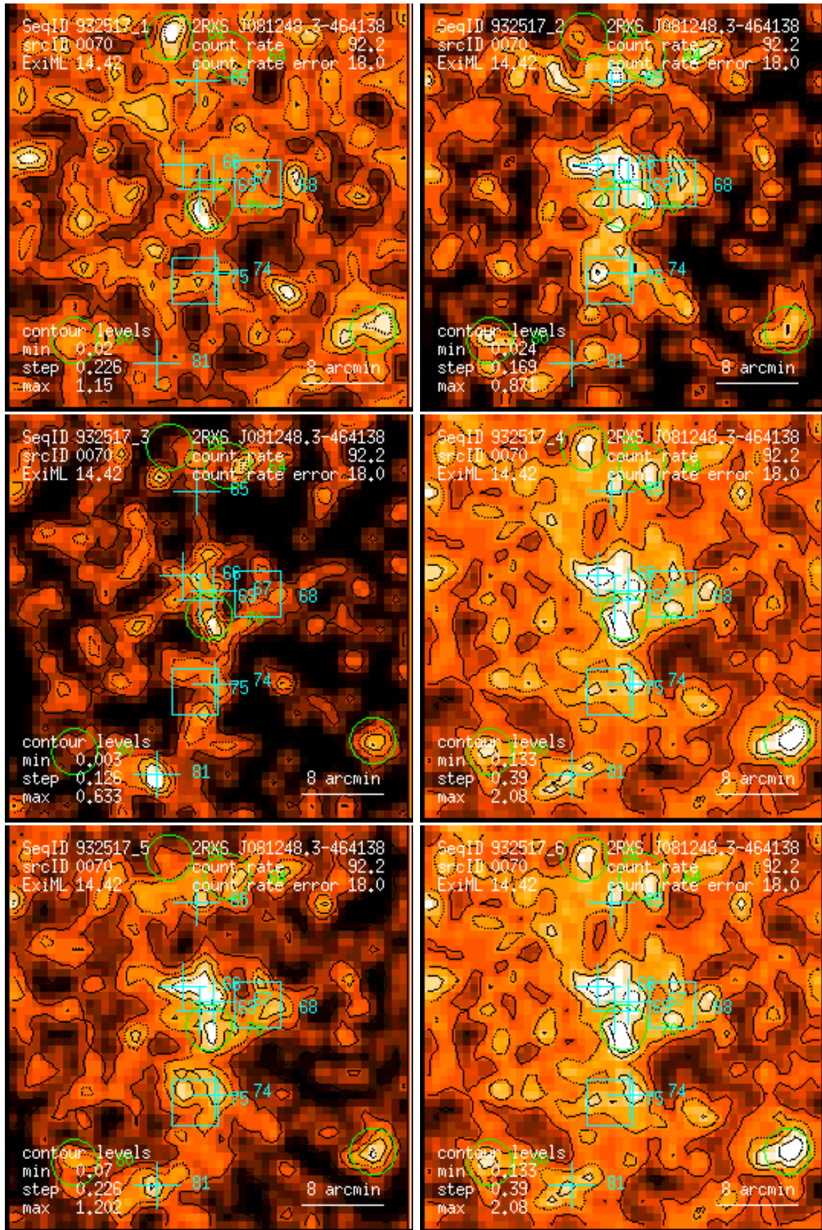
Figure 70: RASS 932517: detection 0070: band rate images, Gaussian filter: (1) PSPC channels 11 – 41, (2) 52 – 90, (3) 91 – 201, (4) 11 – 235, (5) 52 – 201, (6) 11 – 201. Broad band rates in counts/ks. Band rate contour levels in counts/ks/arcmin 2 .
