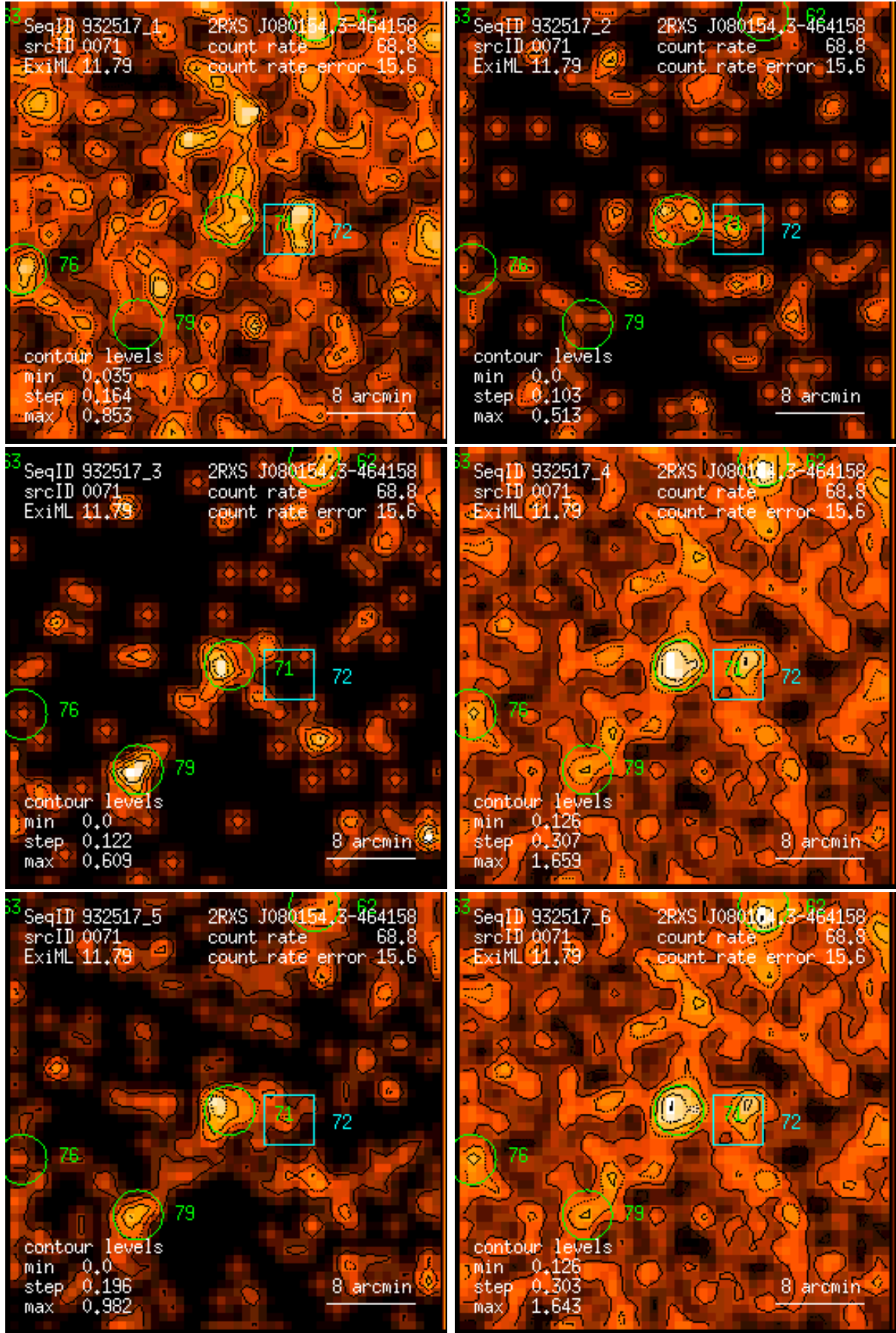
Figure 71: RASS 932517: detection 0071: band rate images, Gaussian filter: (1) PSPC channels 11 – 41, (2) 52 – 90, (3) 91 – 201, (4) 11 – 235, (5) 52 – 201, (6) 11 – 201. Broad band rates in counts/ks. Band rate contour levels in counts/ks/arcmin 2 .
