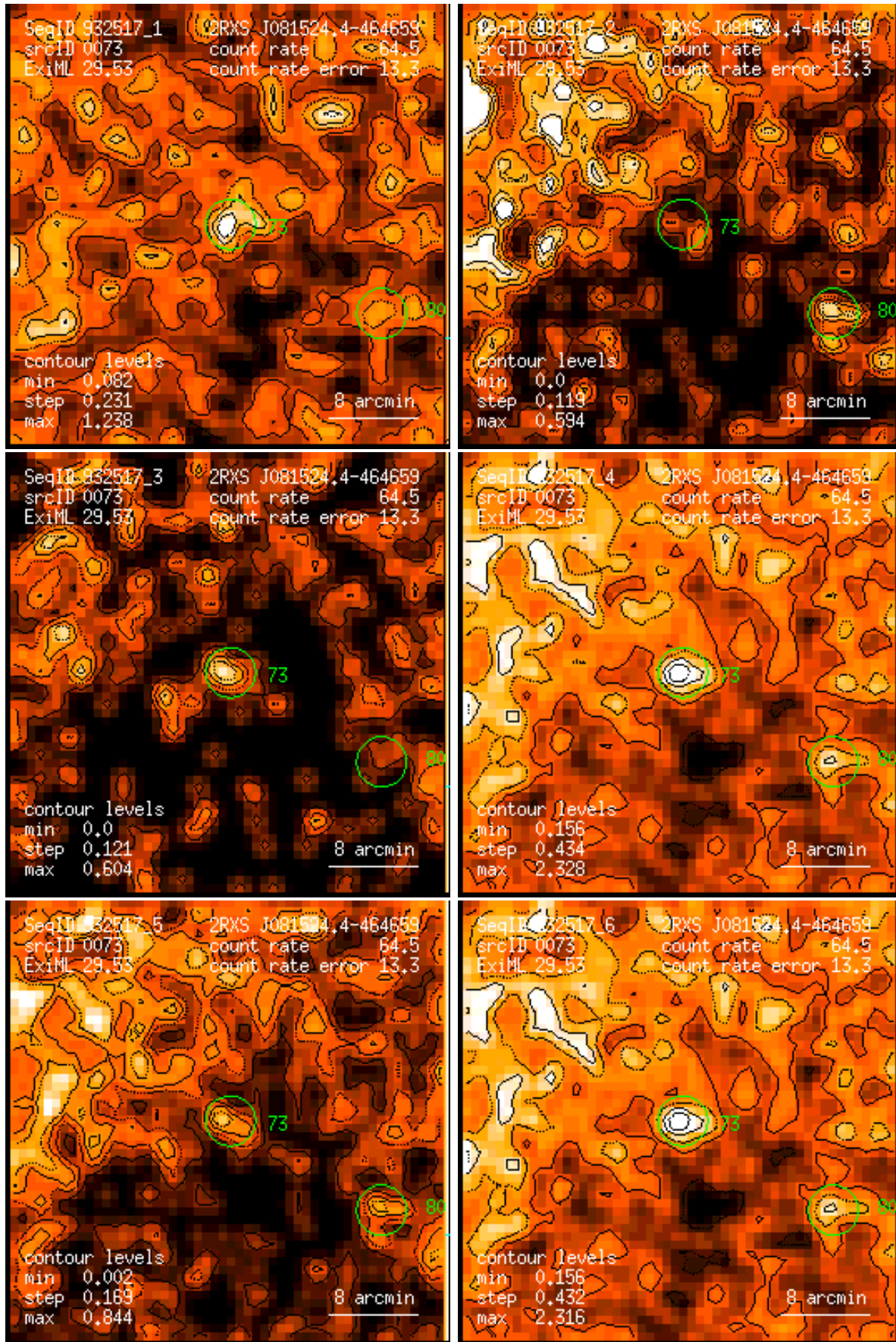
Figure 73: RASS 932517: detection 0073: band rate images, Gaussian filter: (1) PSPC channels 11 – 41, (2) 52 – 90, (3) 91 – 201, (4) 11 – 235, (5) 52 – 201, (6) 11 – 201. Broad band rates in counts/ks. Band rate contour levels in counts/ks/arcmin 2 .
