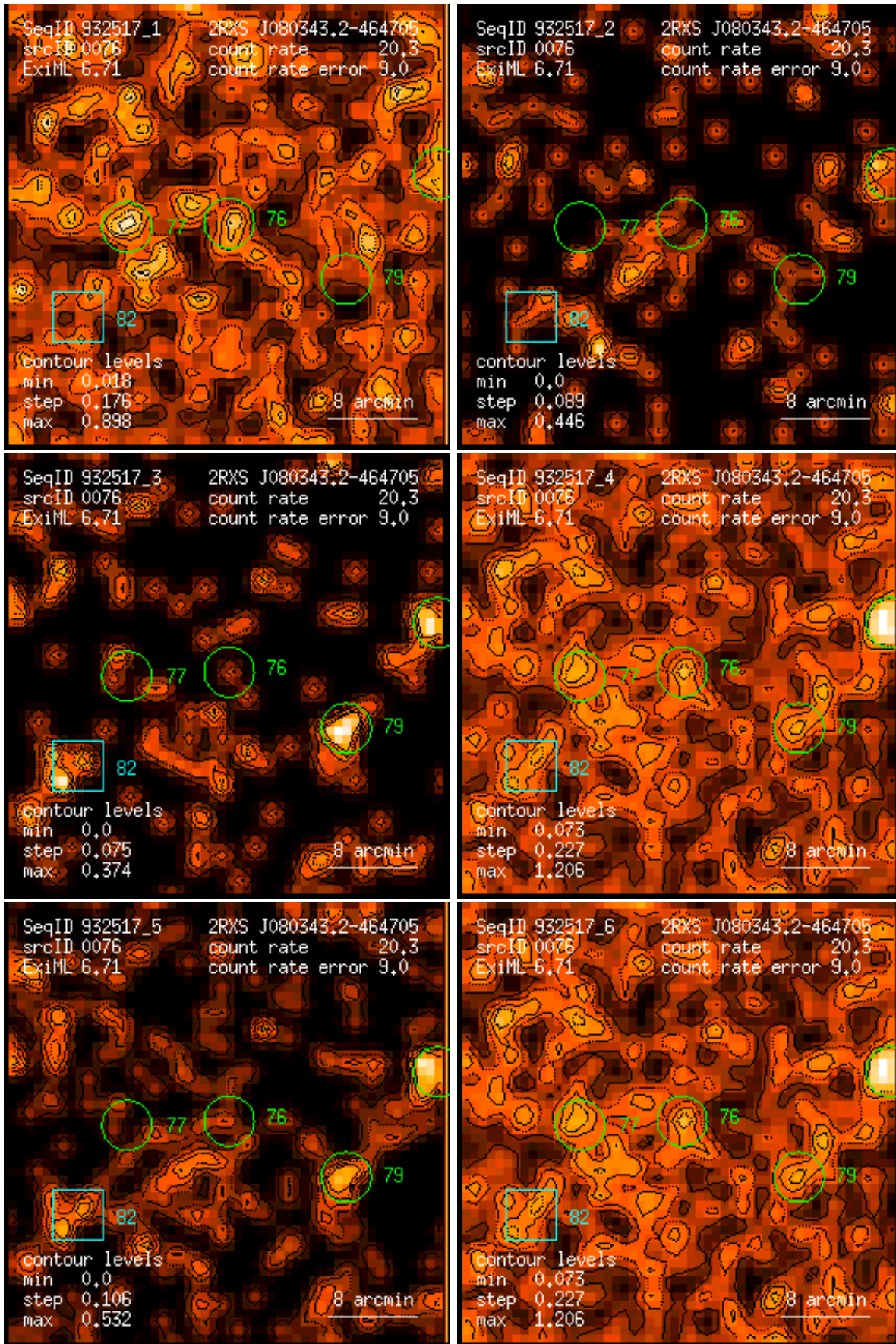
Figure 76: RASS 932517: detection 0076: band rate images, Gaussian filter: (1) PSPC channels 11 – 41, (2) 52 – 90, (3) 91 – 201, (4) 11 – 235, (5) 52 – 201, (6) 11 – 201. Broad band rates in counts/ks. Band rate contour levels in counts/ks/arcmin 2 .
