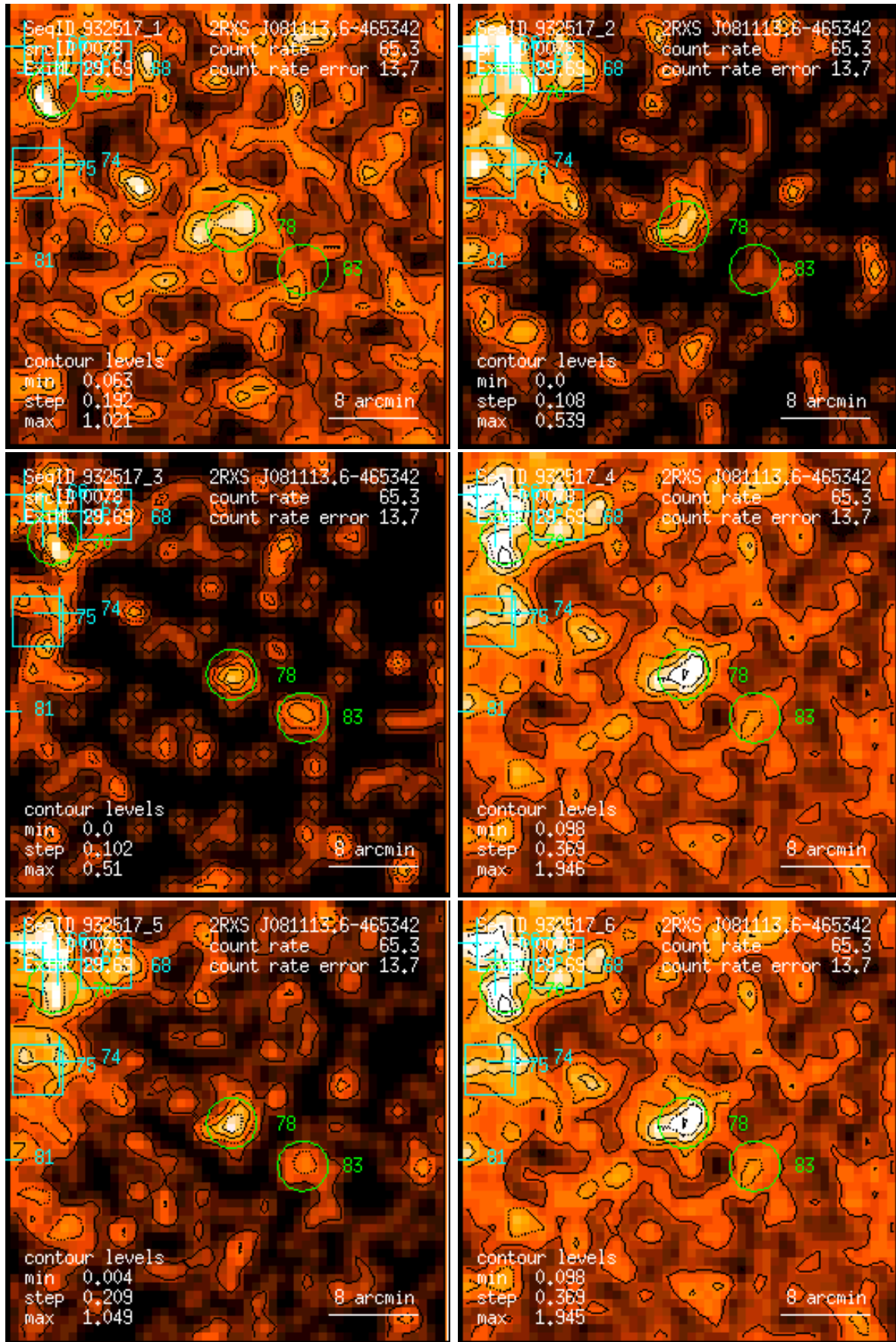
Figure 78: RASS 932517: detection 0078: band rate images, Gaussian filter: (1) PSPC channels 11 – 41, (2) 52 – 90, (3) 91 – 201, (4) 11 – 235, (5) 52 – 201, (6) 11 – 201. Broad band rates in counts/ks. Band rate contour levels in counts/ks/arcmin 2 .
