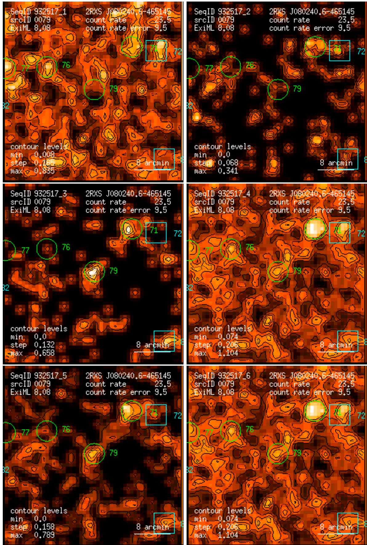
Figure 79: RASS 932517: detection 0079: band rate images, Gaussian filter: (1) PSPC channels 11 – 41, (2) 52 – 90, (3) 91 – 201, (4) 11 – 235, (5) 52 – 201, (6) 11 – 201. Broad band rates in counts/ks. Band rate contour levels in counts/ks/arcmin 2 .
