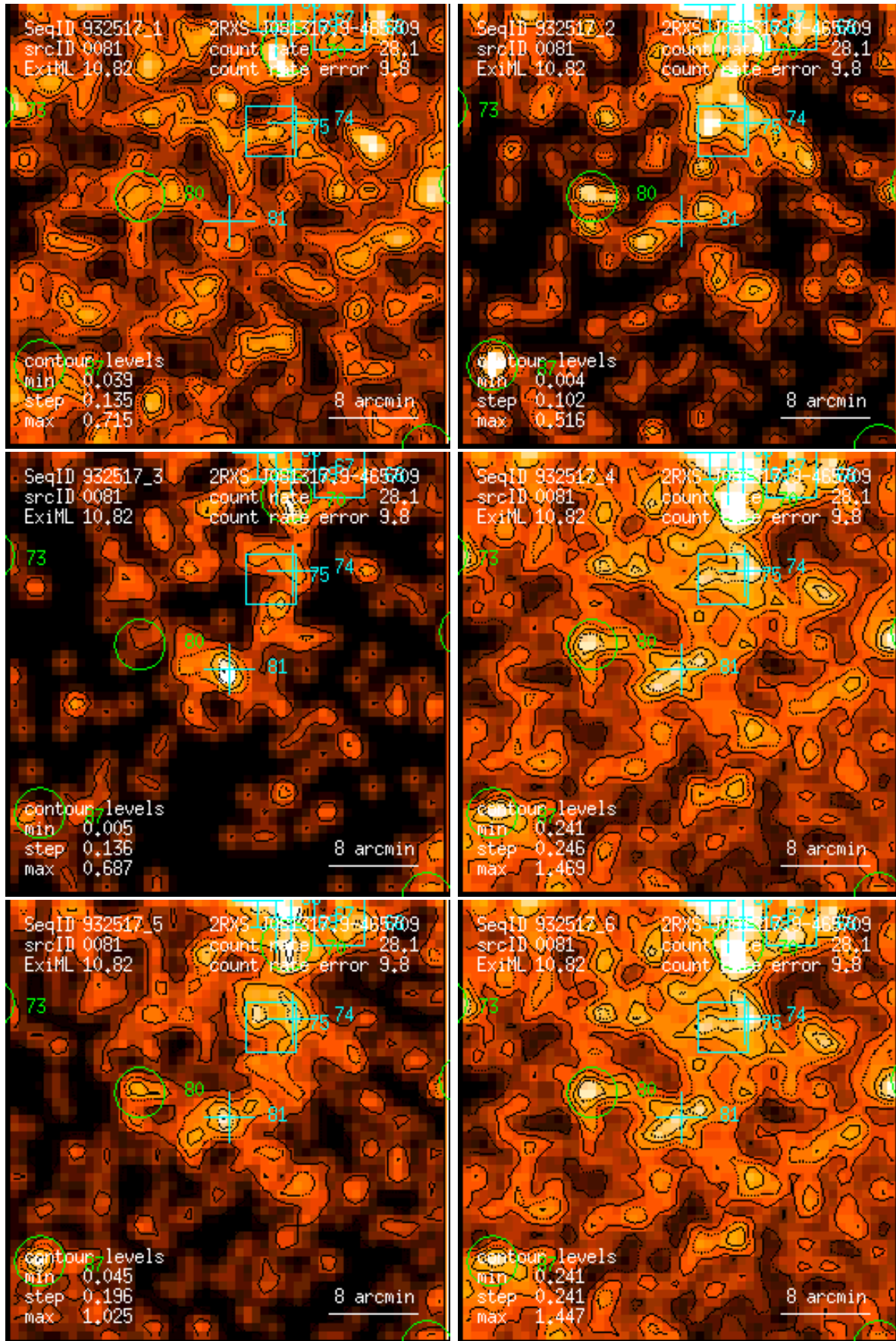
Figure 81: RASS 932517: detection 0081: band rate images, Gaussian filter: (1) PSPC channels 11 – 41, (2) 52 – 90, (3) 91 – 201, (4) 11 – 235, (5) 52 – 201, (6) 11 – 201. Broad band rates in counts/ks. Band rate contour levels in counts/ks/arcmin 2 .
