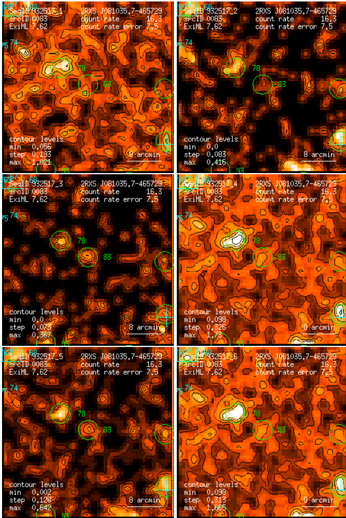
Figure 83: RASS 932517: detection 0083: band rate images, Gaussian filter: (1) PSPC channels 11 – 41, (2) 52 – 90, (3) 91 – 201, (4) 11 – 235, (5) 52 – 201, (6) 11 – 201. Broad band rates in counts/ks. Band rate contour levels in counts/ks/arcmin 2 .
