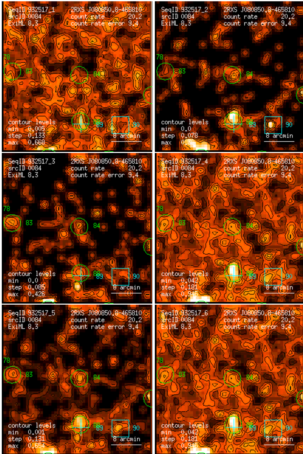
Figure 84: RASS 932517: detection 0084: band rate images, Gaussian filter: (1) PSPC channels 11 – 41, (2) 52 – 90, (3) 91 – 201, (4) 11 – 235, (5) 52 – 201, (6) 11 – 201. Broad band rates in counts/ks. Band rate contour levels in counts/ks/arcmin 2 .
