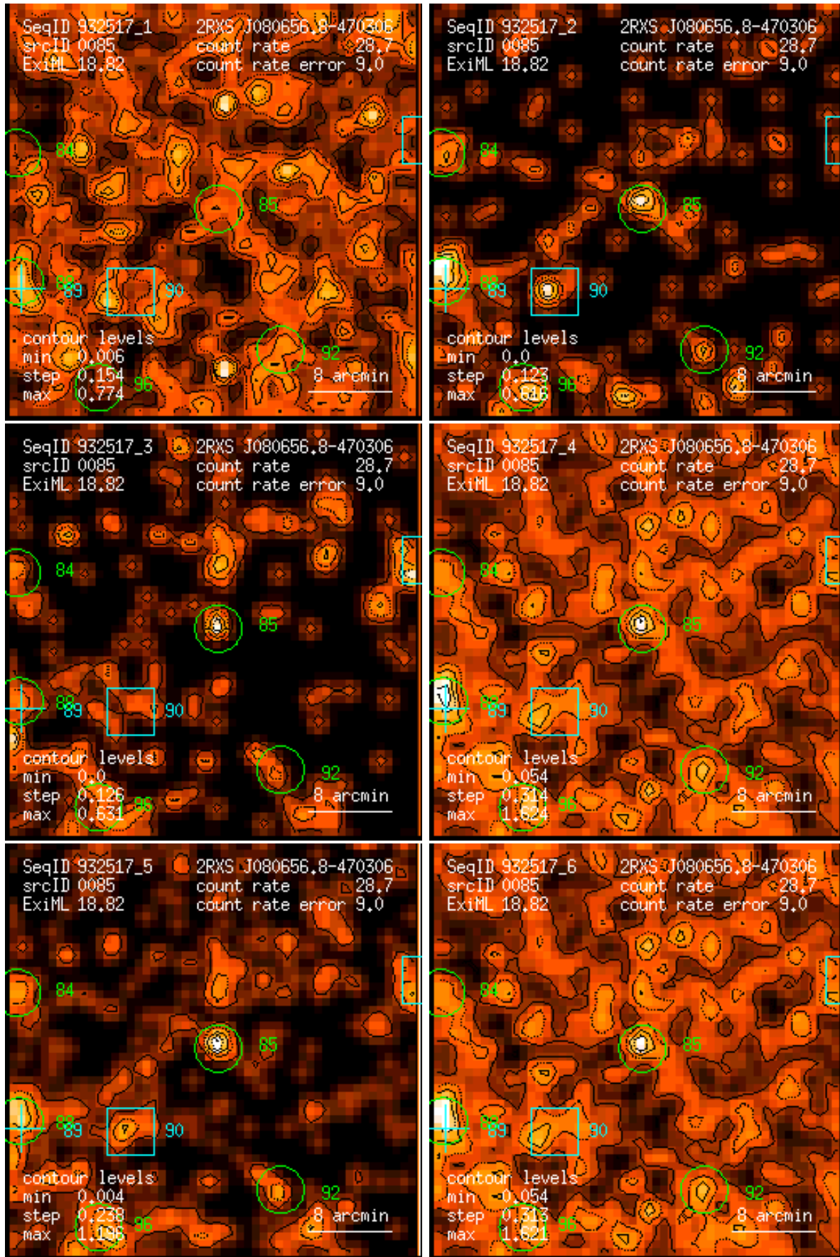
Figure 85: RASS 932517: detection 0085: band rate images, Gaussian filter: (1) PSPC channels 11 – 41, (2) 52 – 90, (3) 91 – 201, (4) 11 – 235, (5) 52 – 201, (6) 11 – 201. Broad band rates in counts/ks. Band rate contour levels in counts/ks/arcmin 2 .
