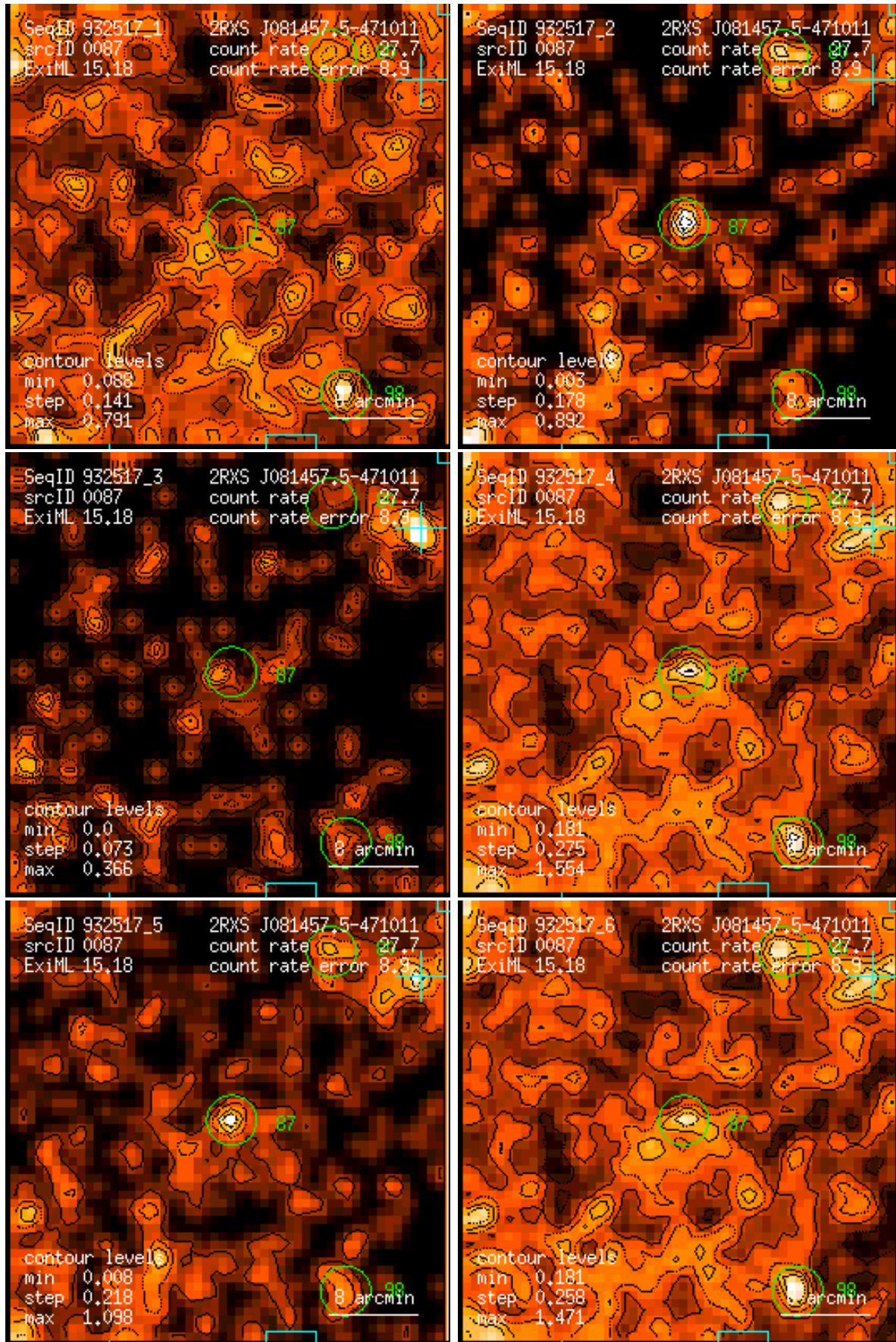
Figure 87: RASS 932517: detection 0087: band rate images, Gaussian filter: (1) PSPC channels 11 – 41, (2) 52 – 90, (3) 91 – 201, (4) 11 – 235, (5) 52 – 201, (6) 11 – 201. Broad band rates in counts/ks. Band rate contour levels in counts/ks/arcmin 2 .
