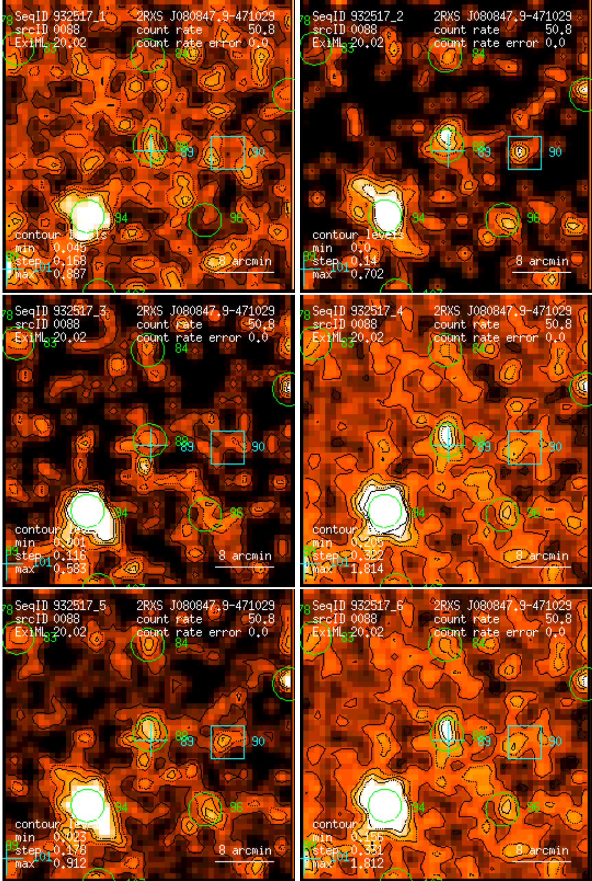
Figure 88: RASS 932517: detection 0088: band rate images, Gaussian filter: (1) PSPC channels 11 – 41, (2) 52 – 90, (3) 91 – 201, (4) 11 – 235, (5) 52 – 201, (6) 11 – 201. Broad band rates in counts/ks. Band rate contour levels in counts/ks/arcmin 2 .
