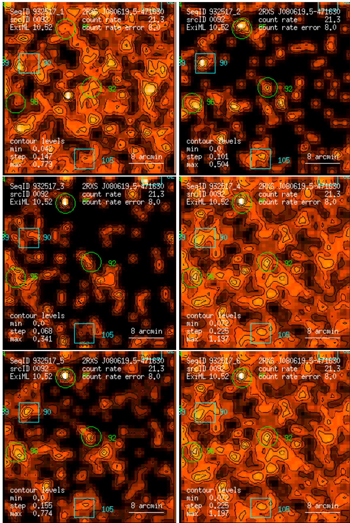
Figure 92: RASS 932517: detection 0092: band rate images, Gaussian filter: (1) PSPC channels 11 – 41, (2) 52 – 90, (3) 91 – 201, (4) 11 – 235, (5) 52 – 201, (6) 11 – 201. Broad band rates in counts/ks. Band rate contour levels in counts/ks/arcmin 2 .
