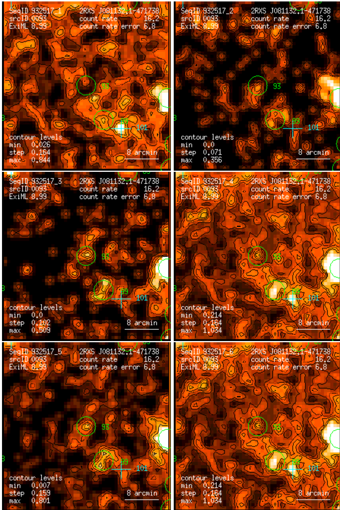
Figure 93: RASS 932517: detection 0093: band rate images, Gaussian filter: (1) PSPC channels 11 – 41, (2) 52 – 90, (3) 91 – 201, (4) 11 – 235, (5) 52 – 201, (6) 11 – 201. Broad band rates in counts/ks. Band rate contour levels in counts/ks/arcmin 2 .
