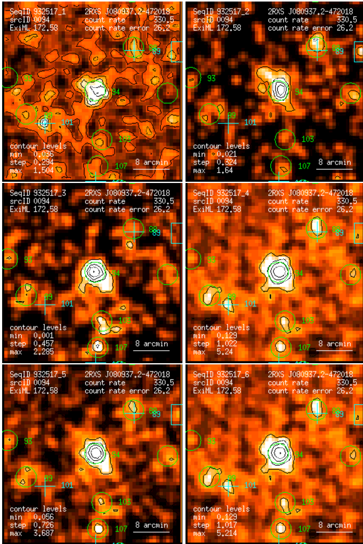
Figure 94: RASS 932517: detection 0094: band rate images, Gaussian filter: (1) PSPC channels 11 – 41, (2) 52 – 90, (3) 91 – 201, (4) 11 – 235, (5) 52 – 201, (6) 11 – 201. Broad band rates in counts/ks. Band rate contour levels in counts/ks/arcmin 2 .
