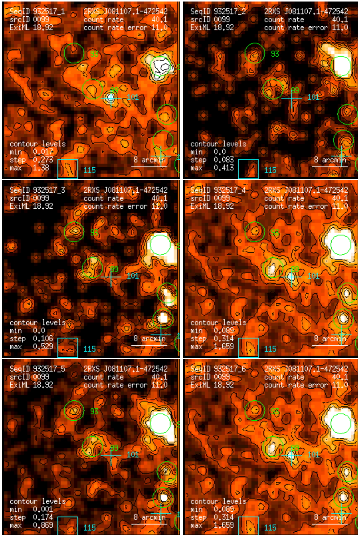
Figure 99: RASS 932517: detection 0099: band rate images, Gaussian filter: (1) PSPC channels 11 – 41, (2) 52 – 90, (3) 91 – 201, (4) 11 – 235, (5) 52 – 201, (6) 11 – 201. Broad band rates in counts/ks. Band rate contour levels in counts/ks/arcmin 2 .
