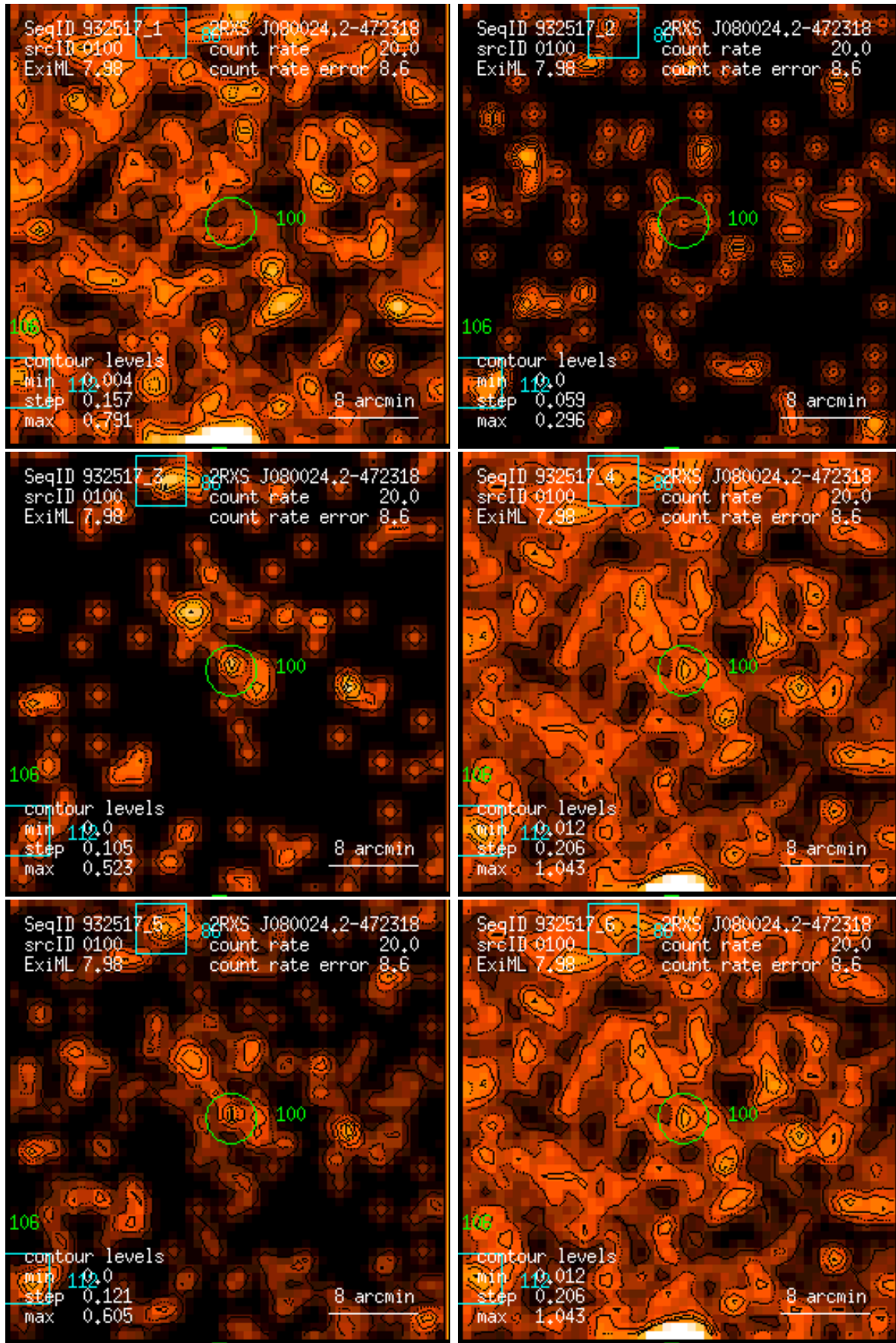
Figure 100: RASS 932517: detection 0100: band rate images, Gaussian filter: (1) PSPC channels 11 – 41, (2) 52 – 90, (3) 91 – 201, (4) 11 – 235, (5) 52 – 201, (6) 11 – 201. Broad band rates in counts/ks. Band rate contour levels in counts/ks/arcmin 2 .
