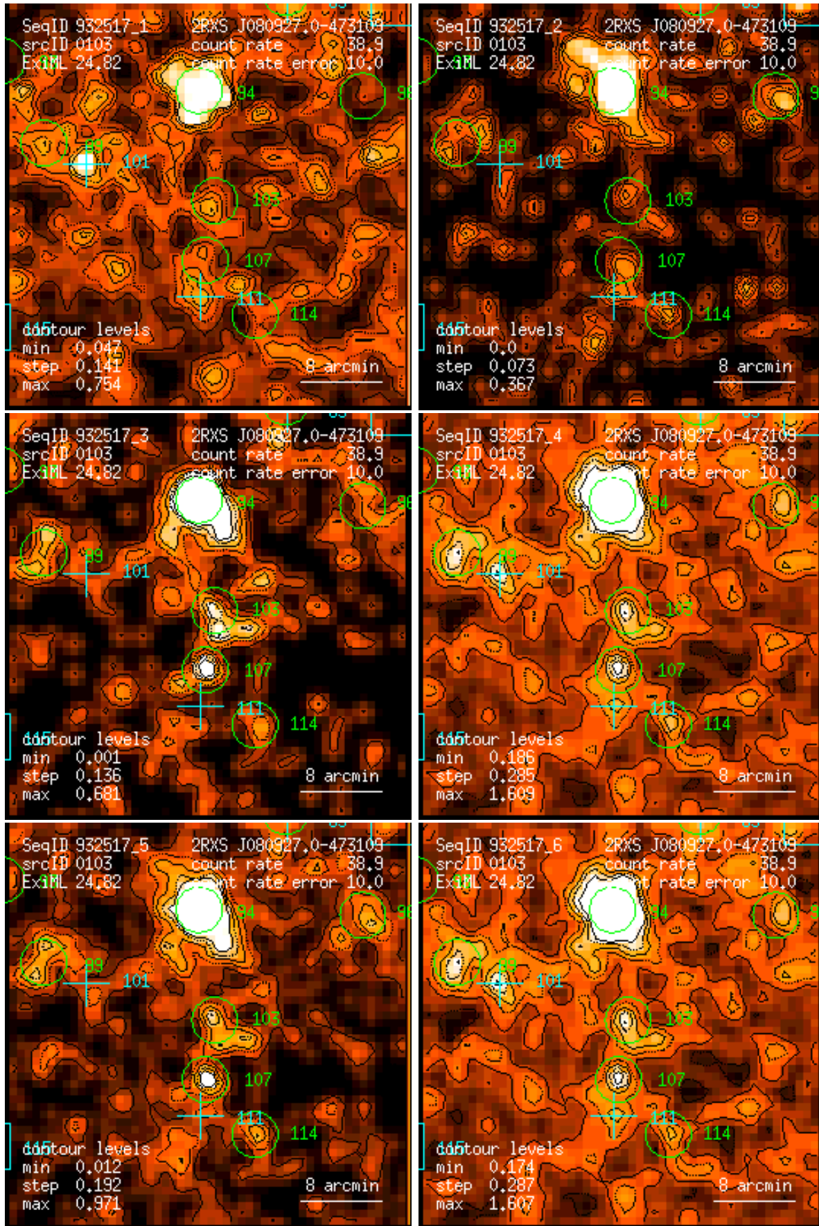
Figure 103: RASS 932517: detection 0103: band rate images, Gaussian filter: (1) PSPC channels 11 – 41, (2) 52 – 90, (3) 91 – 201, (4) 11 – 235, (5) 52 – 201, (6) 11 – 201. Broad band rates in counts/ks. Band rate contour levels in counts/ks/arcmin 2 .
