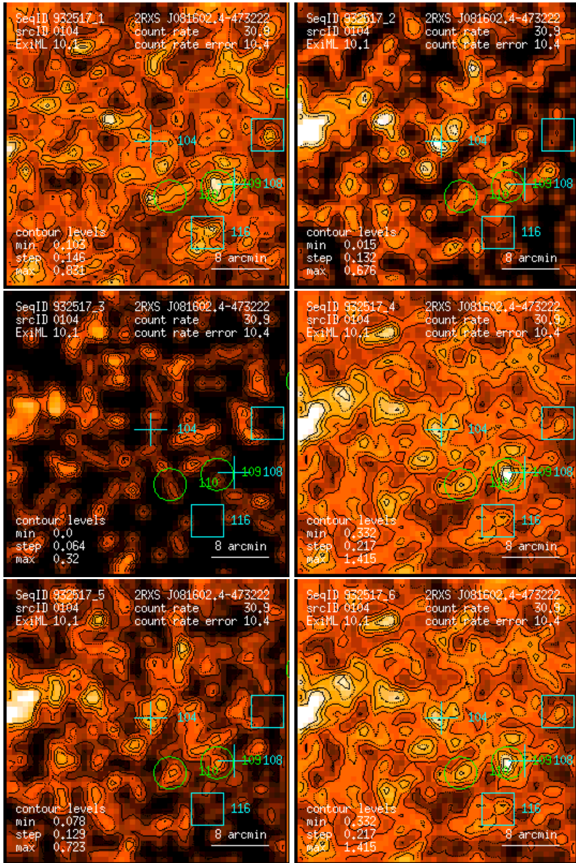
Figure 104: RASS 932517: detection 0104: band rate images, Gaussian filter: (1) PSPC channels 11 – 41, (2) 52 – 90, (3) 91 – 201, (4) 11 – 235, (5) 52 – 201, (6) 11 – 201. Broad band rates in counts/ks. Band rate contour levels in counts/ks/arcmin 2 .
