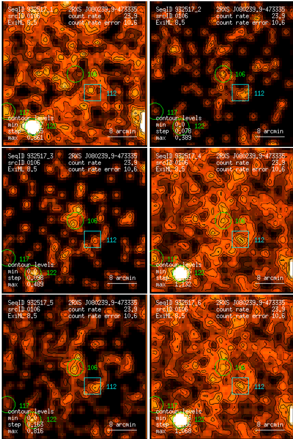
Figure 106: RASS 932517: detection 0106: band rate images, Gaussian filter: (1) PSPC channels 11 – 41, (2) 52 – 90, (3) 91 – 201, (4) 11 – 235, (5) 52 – 201, (6) 11 – 201. Broad band rates in counts/ks. Band rate contour levels in counts/ks/arcmin 2 .
