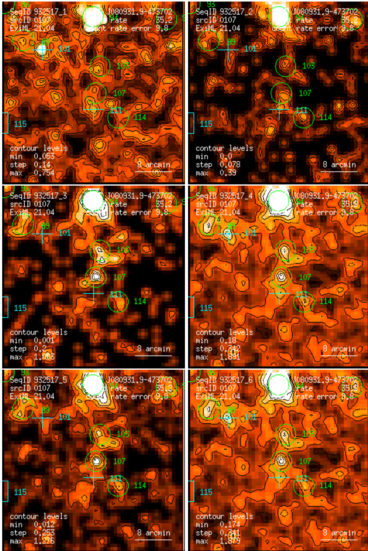
Figure 107: RASS 932517: detection 0107: band rate images, Gaussian filter: (1) PSPC channels 11 – 41, (2) 52 – 90, (3) 91 – 201, (4) 11 – 235, (5) 52 – 201, (6) 11 – 201. Broad band rates in counts/ks. Band rate contour levels in counts/ks/arcmin 2 .
