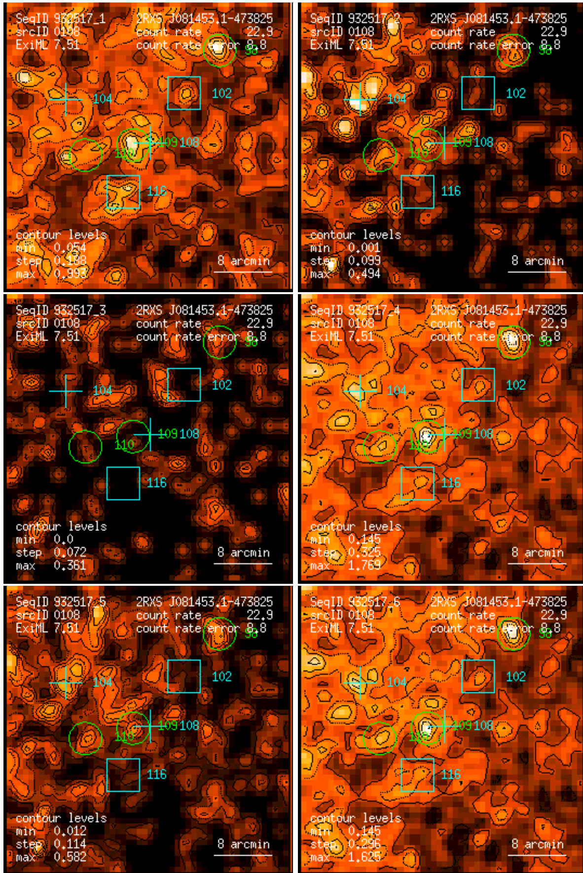
Figure 108: RASS 932517: detection 0108: band rate images, Gaussian filter: (1) PSPC channels 11 – 41, (2) 52 – 90, (3) 91 – 201, (4) 11 – 235, (5) 52 – 201, (6) 11 – 201. Broad band rates in counts/ks. Band rate contour levels in counts/ks/arcmin 2 .
