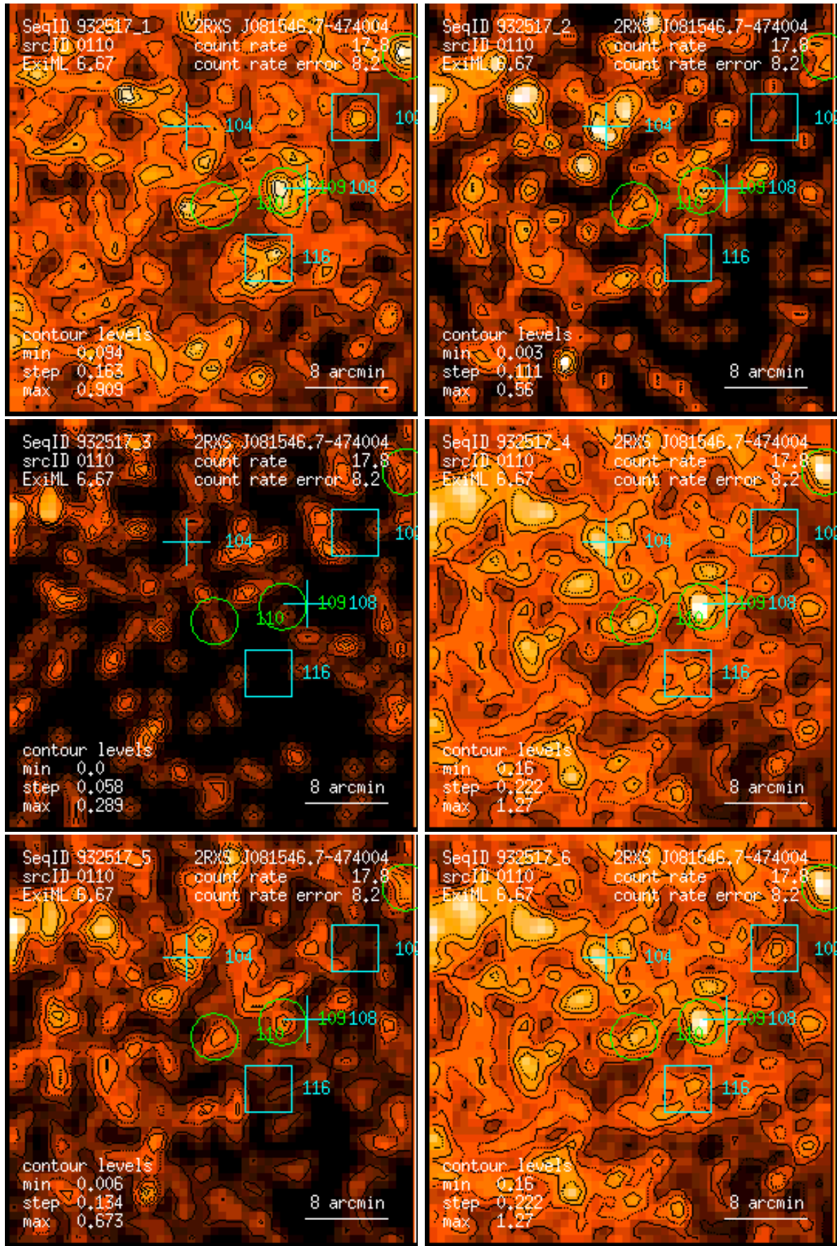
Figure 110: RASS 932517: detection 0110: band rate images, Gaussian filter: (1) PSPC channels 11 – 41, (2) 52 – 90, (3) 91 – 201, (4) 11 – 235, (5) 52 – 201, (6) 11 – 201. Broad band rates in counts/ks. Band rate contour levels in counts/ks/arcmin 2 .
