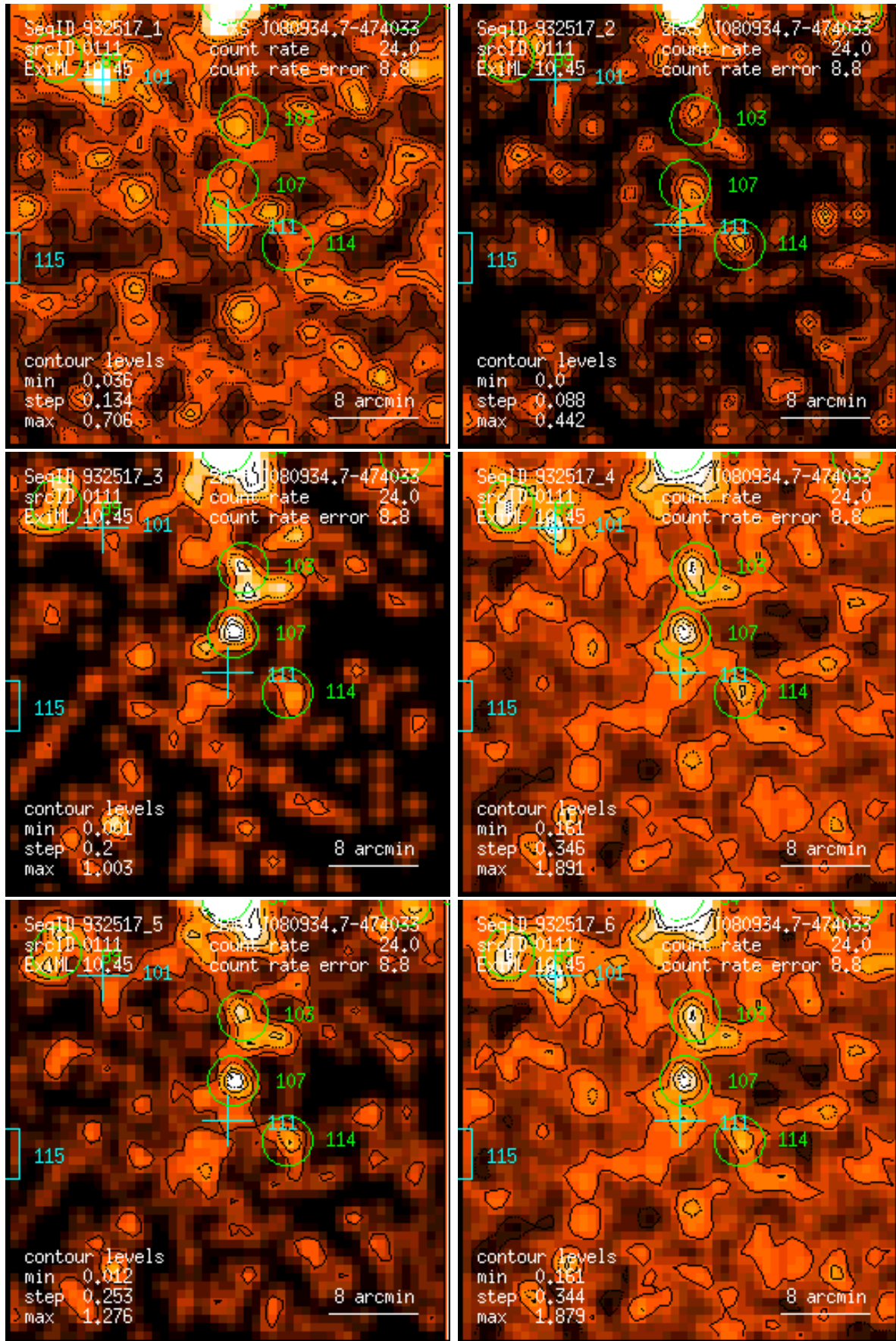
Figure 111: RASS 932517: detection 0111: band rate images, Gaussian filter: (1) PSPC channels 11 – 41, (2) 52 – 90, (3) 91 – 201, (4) 11 – 235, (5) 52 – 201, (6) 11 – 201. Broad band rates in counts/ks. Band rate contour levels in counts/ks/arcmin 2 .
