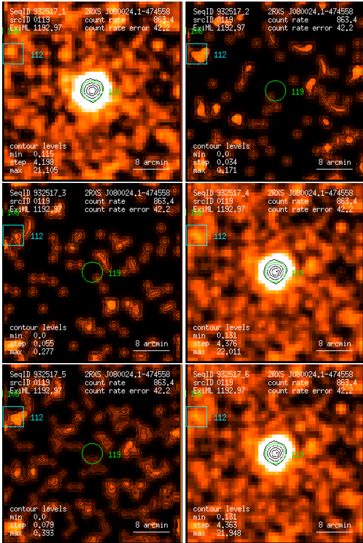
Figure 119: RASS 932517: detection 0119: band rate images, Gaussian filter: (1) PSPC channels 11 – 41, (2) 52 – 90, (3) 91 – 201, (4) 11 – 235, (5) 52 – 201, (6) 11 – 201. Broad band rates in counts/ks. Band rate contour levels in counts/ks/arcmin 2 .
