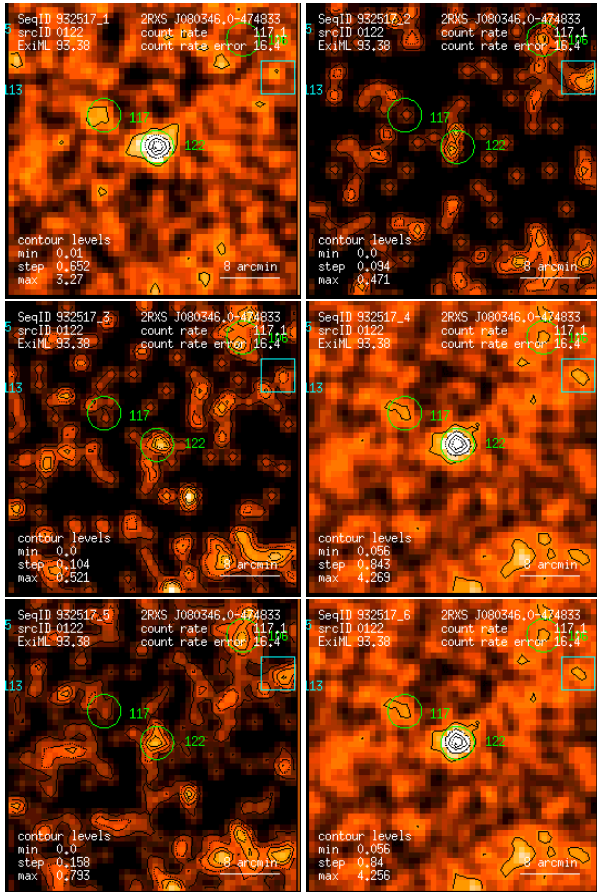
Figure 122: RASS 932517: detection 0122: band rate images, Gaussian filter: (1) PSPC channels 11 – 41, (2) 52 – 90, (3) 91 – 201, (4) 11 – 235, (5) 52 – 201, (6) 11 – 201. Broad band rates in counts/ks. Band rate contour levels in counts/ks/arcmin 2 .
