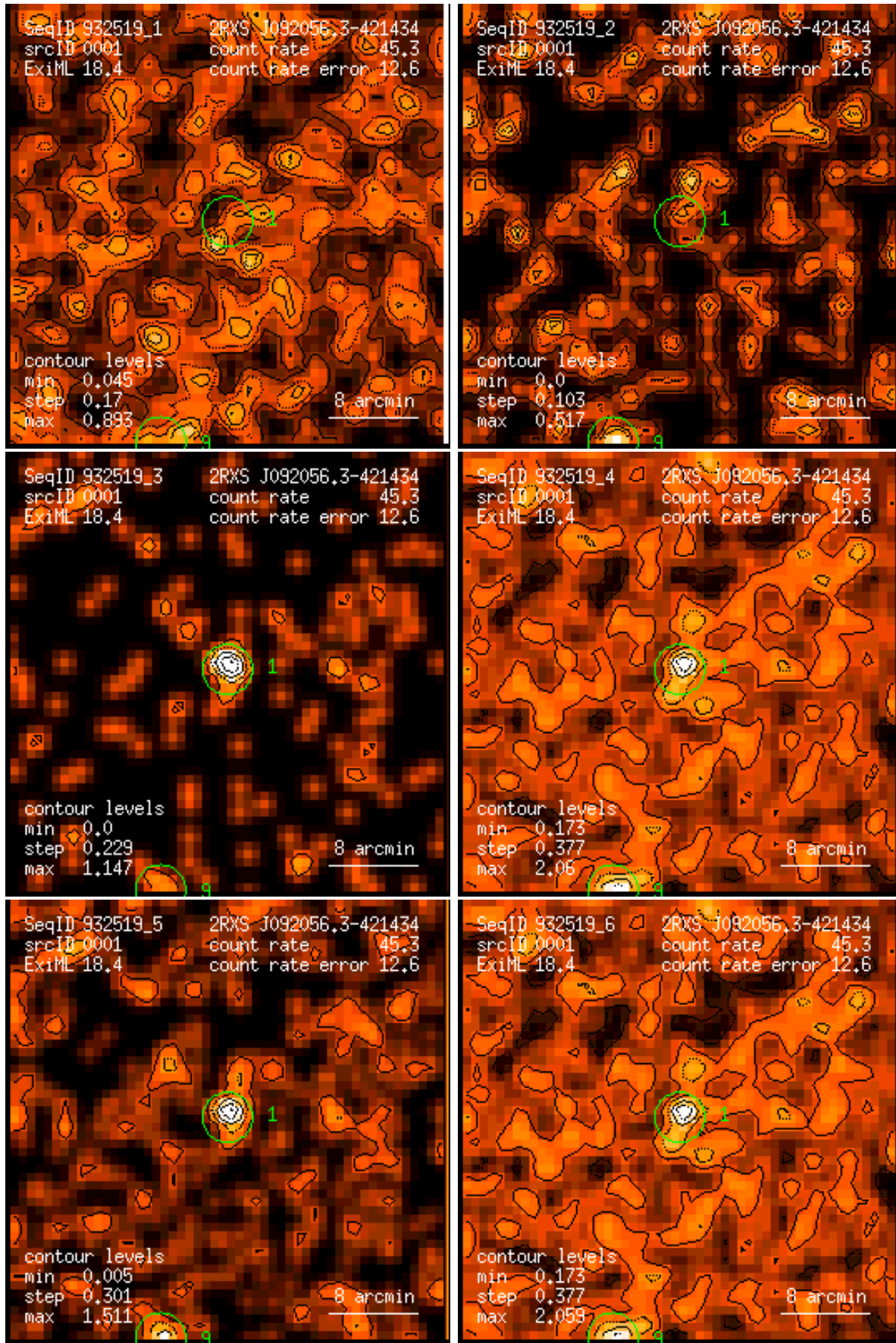
Figure 1: RASS 932519: detection 0001: band rate images, Gaussian filter: (1) PSPC channels 11 – 41, (2) 52 – 90, (3) 91 – 201, (4) 11 – 235, (5) 52 – 201, (6) 11 – 201. Broad band rates in counts/ks. Band rate contour levels in counts/ks/arcmin 2 .
