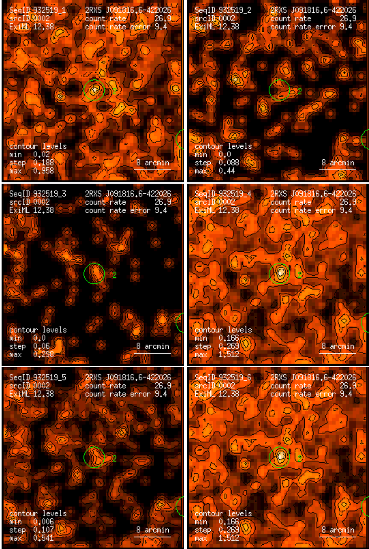
Figure 2: RASS 932519: detection 0002: band rate images, Gaussian filter: (1) PSPC channels 11 – 41, (2) 52 – 90, (3) 91 – 201, (4) 11 – 235, (5) 52 – 201, (6) 11 – 201. Broad band rates in counts/ks. Band rate contour levels in counts/ks/arcmin 2 .
