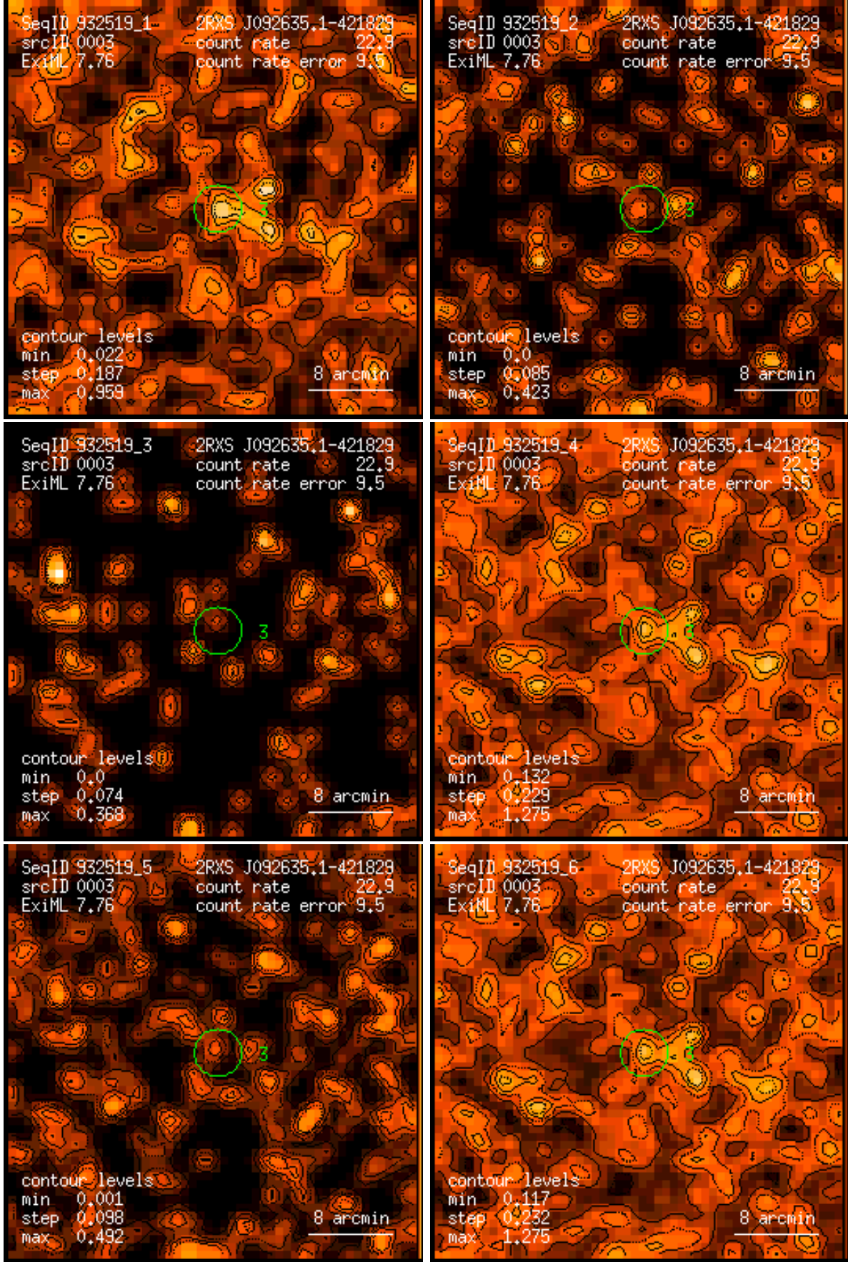
Figure 3: RASS 932519: detection 0003: band rate images, Gaussian filter: (1) PSPC channels 11 – 41, (2) 52 – 90, (3) 91 – 201, (4) 11 – 235, (5) 52 – 201, (6) 11 – 201. Broad band rates in counts/ks. Band rate contour levels in counts/ks/arcmin 2 .
