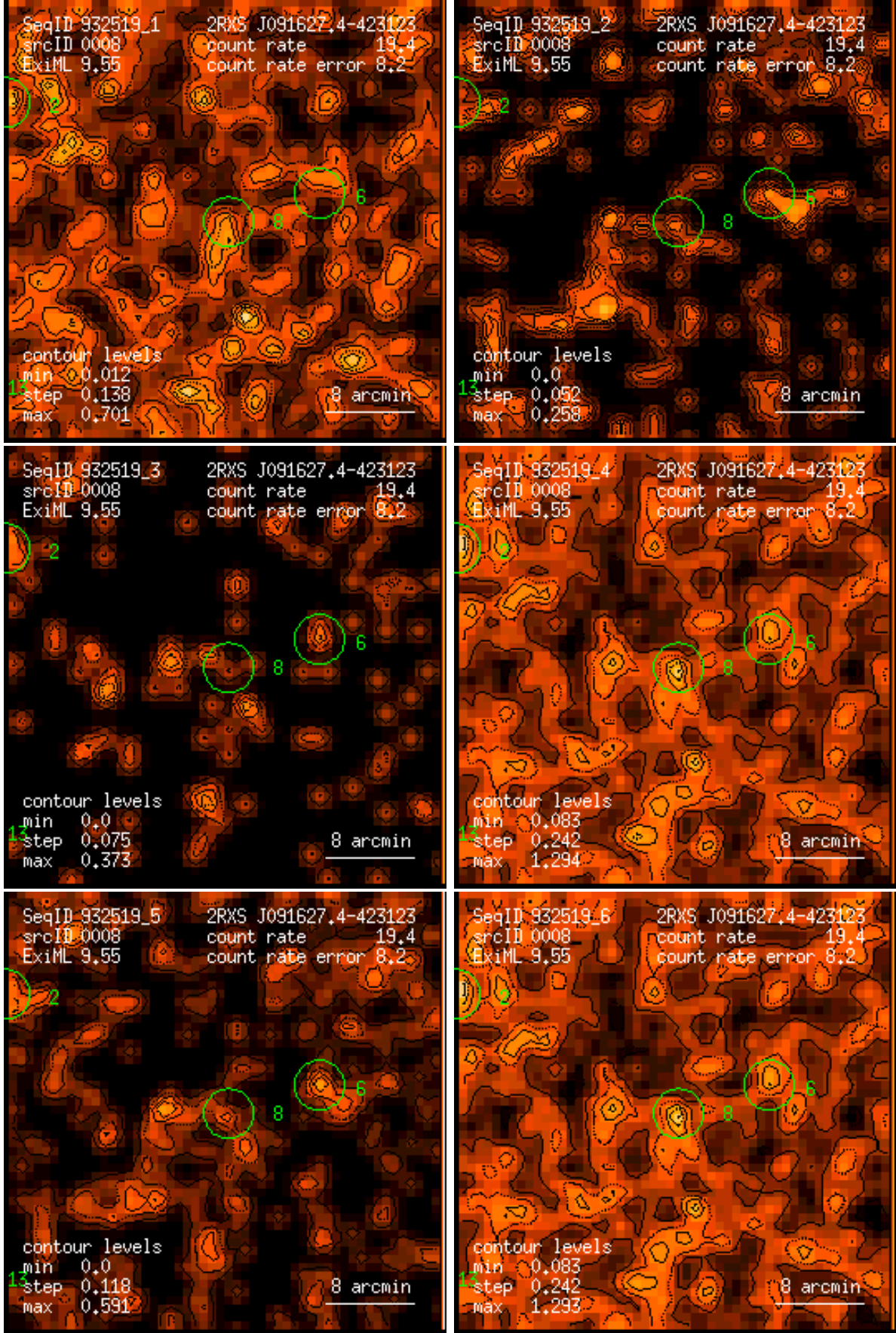
Figure 8: RASS 932519: detection 0008: band rate images, Gaussian filter: (1) PSPC channels 11 – 41, (2) 52 – 90, (3) 91 – 201, (4) 11 – 235, (5) 52 – 201, (6) 11 – 201. Broad band rates in counts/ks. Band rate contour levels in counts/ks/arcmin 2 .
