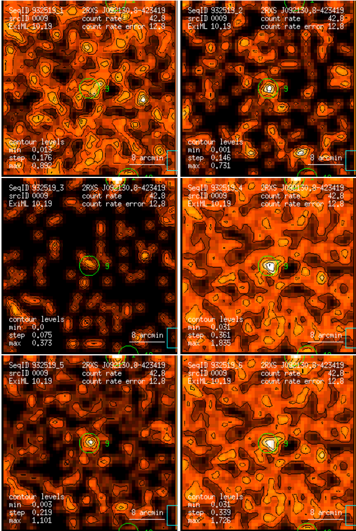
Figure 9: RASS 932519: detection 0009: band rate images, Gaussian filter: (1) PSPC channels 11 – 41, (2) 52 – 90, (3) 91 – 201, (4) 11 – 235, (5) 52 – 201, (6) 11 – 201. Broad band rates in counts/ks. Band rate contour levels in counts/ks/arcmin 2 .
