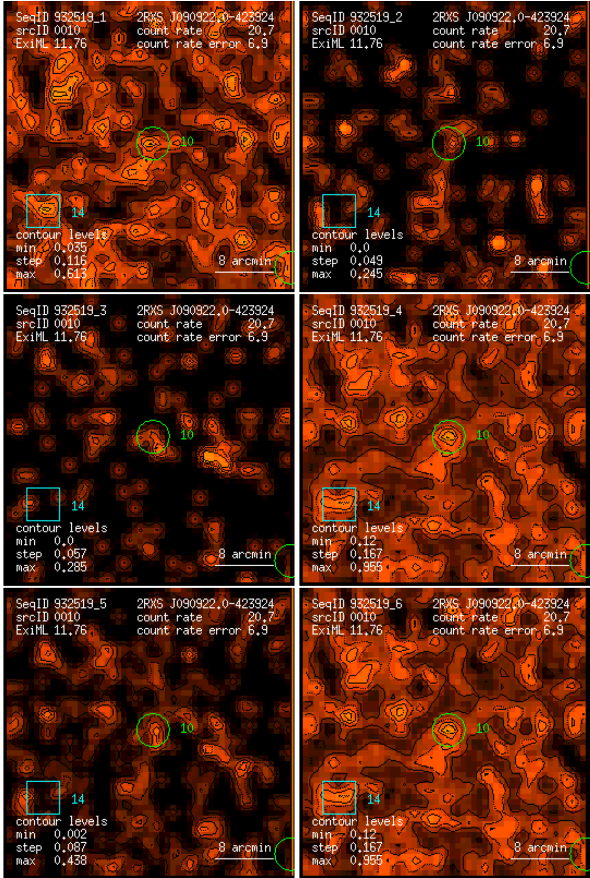
Figure 10: RASS 932519: detection 0010: band rate images, Gaussian filter: (1) PSPC channels 11 – 41, (2) 52 – 90, (3) 91 – 201, (4) 11 – 235, (5) 52 – 201, (6) 11 – 201. Broad band rates in counts/ks. Band rate contour levels in counts/ks/arcmin 2 .
