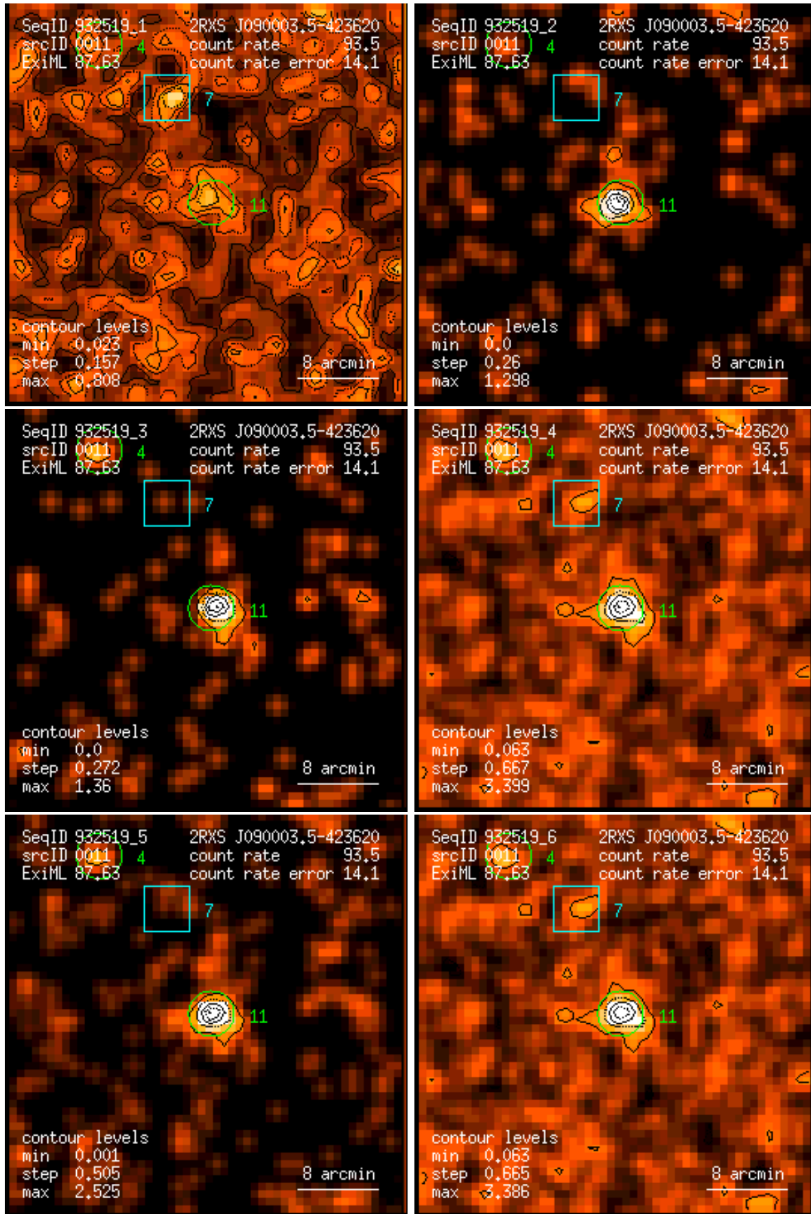
Figure 11: RASS 932519: detection 0011: band rate images, Gaussian filter: (1) PSPC channels 11 – 41, (2) 52 – 90, (3) 91 – 201, (4) 11 – 235, (5) 52 – 201, (6) 11 – 201. Broad band rates in counts/ks. Band rate contour levels in counts/ks/arcmin 2 .
