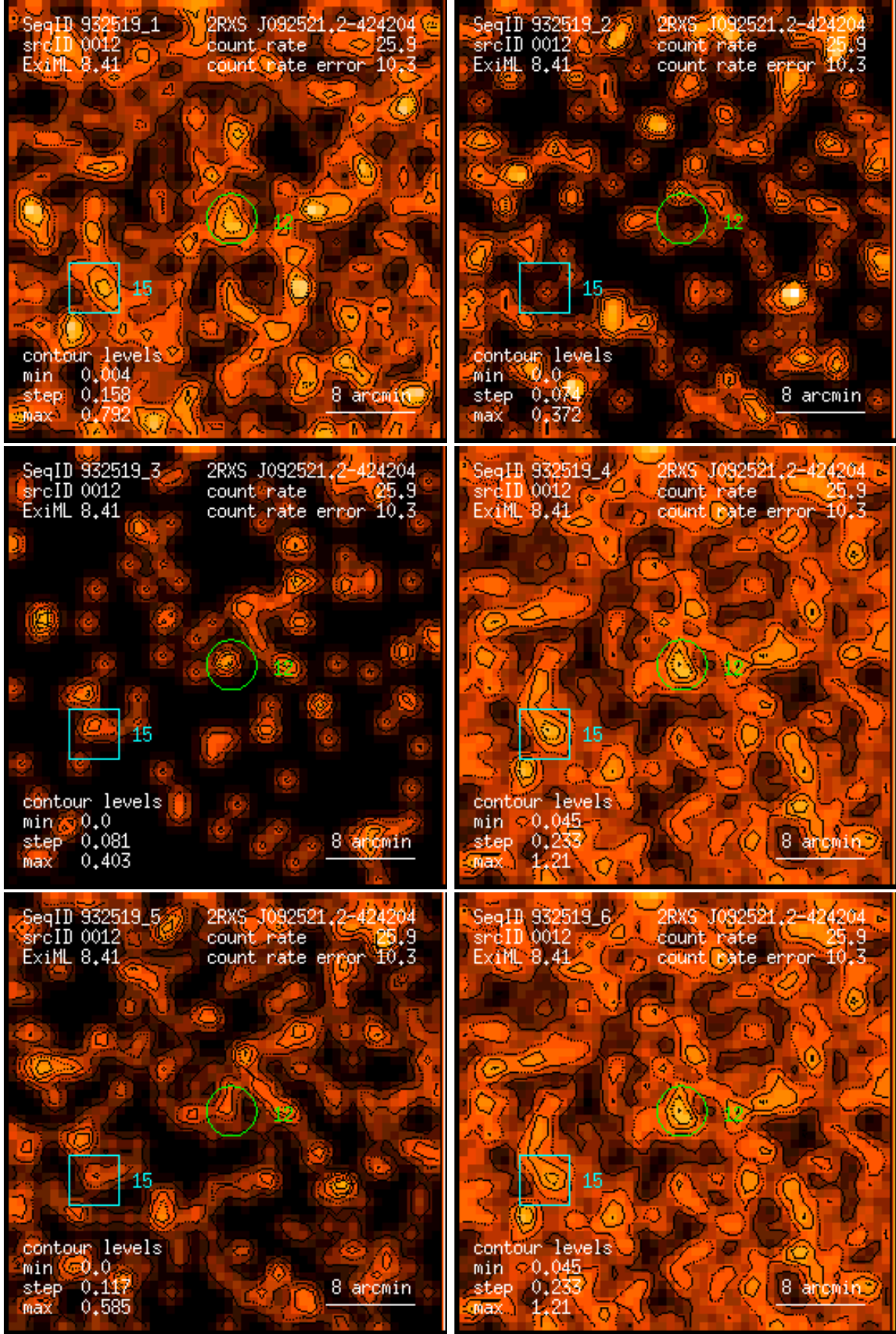
Figure 12: RASS 932519: detection 0012: band rate images, Gaussian filter: (1) PSPC channels 11 – 41, (2) 52 – 90, (3) 91 – 201, (4) 11 – 235, (5) 52 – 201, (6) 11 – 201. Broad band rates in counts/ks. Band rate contour levels in counts/ks/arcmin 2 .
