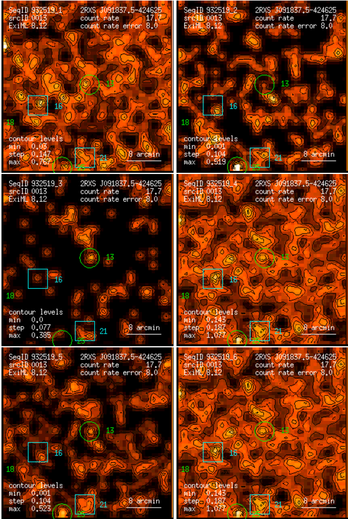
Figure 13: RASS 932519: detection 0013: band rate images, Gaussian filter: (1) PSPC channels 11 – 41, (2) 52 – 90, (3) 91 – 201, (4) 11 – 235, (5) 52 – 201, (6) 11 – 201. Broad band rates in counts/ks. Band rate contour levels in counts/ks/arcmin 2 .
