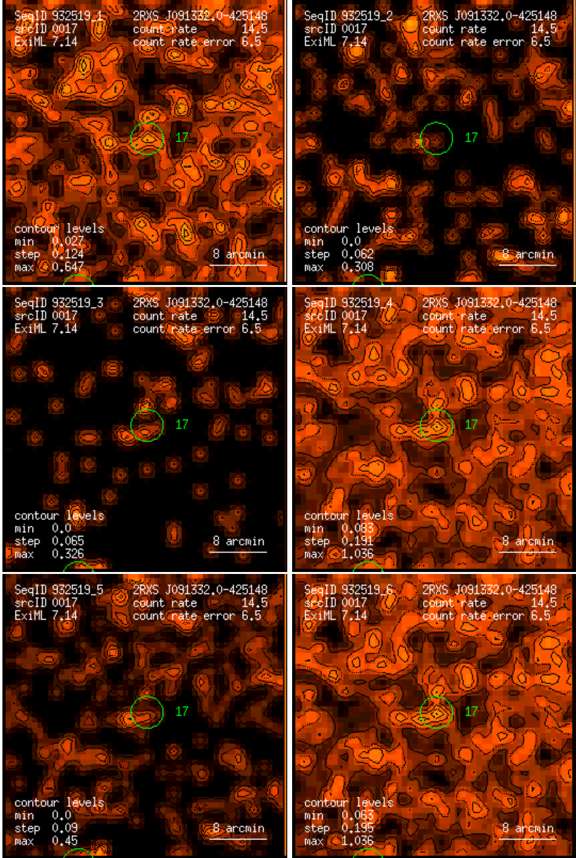
Figure 17: RASS 932519: detection 0017: band rate images, Gaussian filter: (1) PSPC channels 11 – 41, (2) 52 – 90, (3) 91 – 201, (4) 11 – 235, (5) 52 – 201, (6) 11 – 201. Broad band rates in counts/ks. Band rate contour levels in counts/ks/arcmin 2 .
